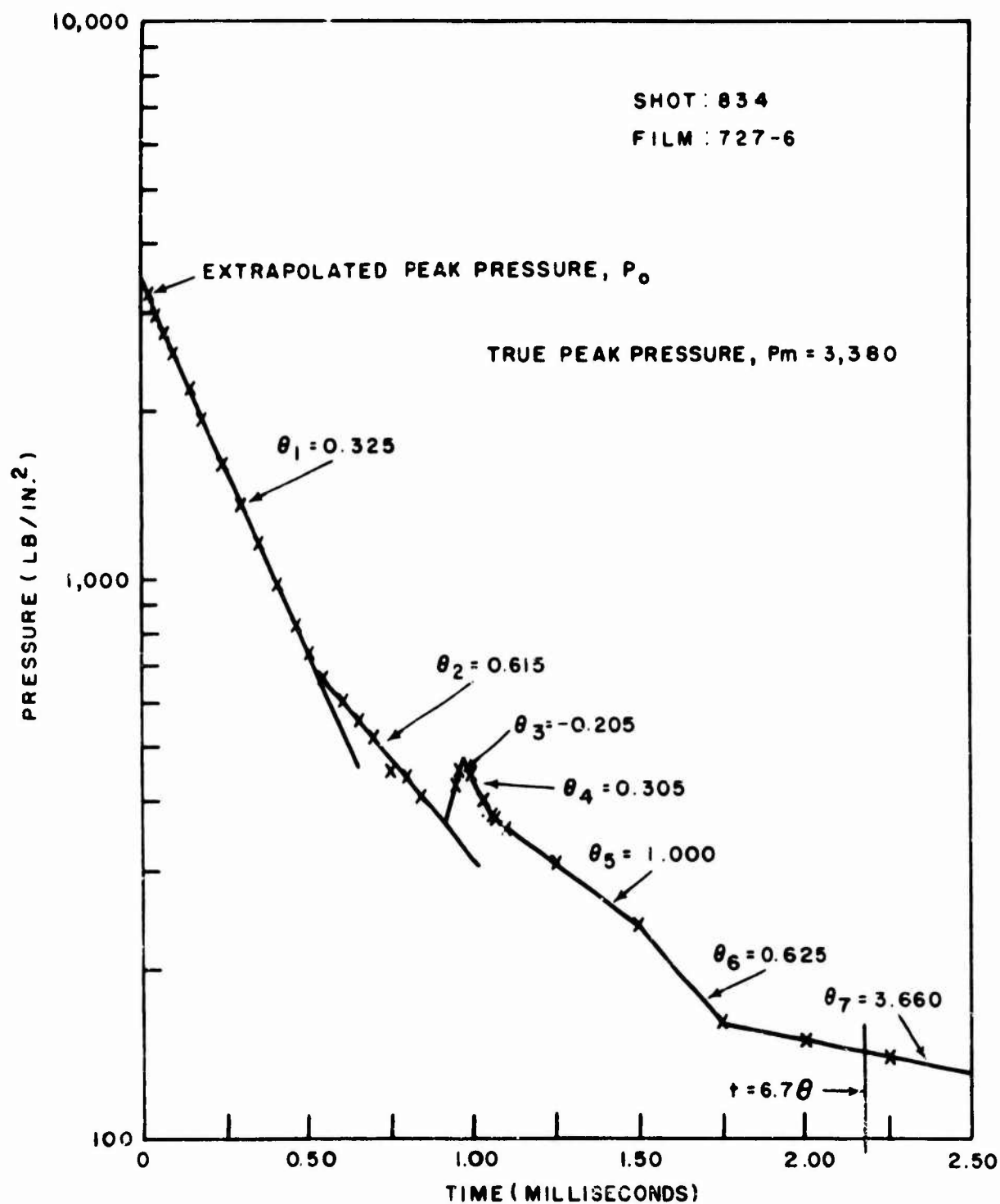
FIG. 2 SEMI-LOG REPRESENTATION OF PRESSURE-TIME RECORD
