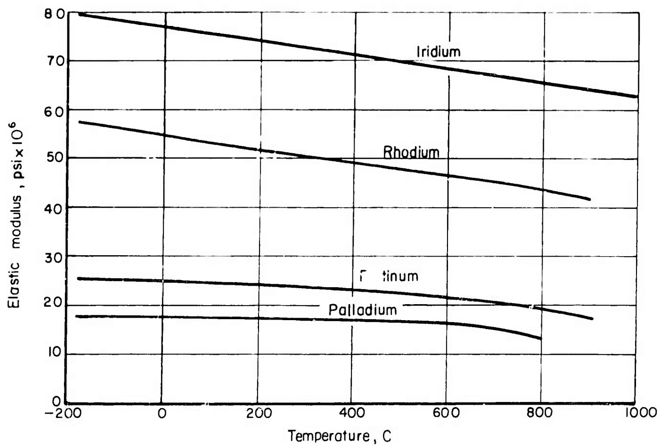
FIGURE 5. EFFECT OF TEMPERATURE ON THE ELASTIC MODULUS OF THE PLATINUM METALS (22)
