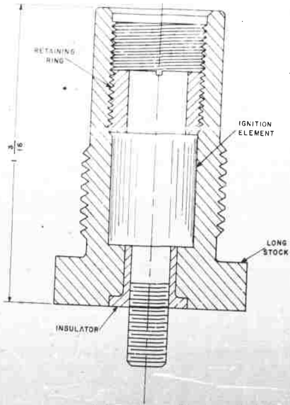
FIG. 30 LONG STOCK ASSEMBLY
