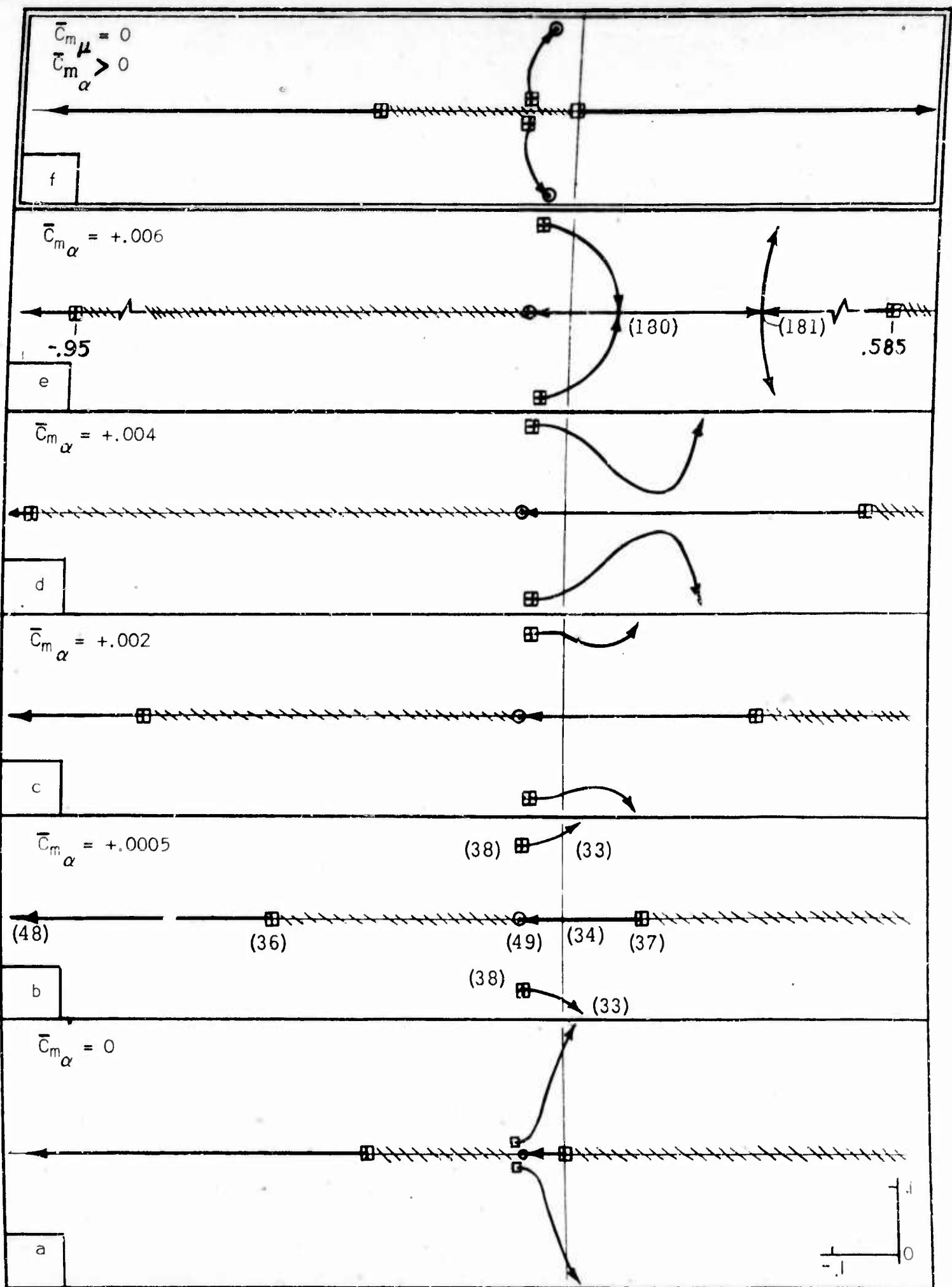
FIGURE 13 - I ROOT LOCUS S.C.D. \mu_r = 0.05 V = 18\text{MPH} \bar{C}_m \mu > 0
