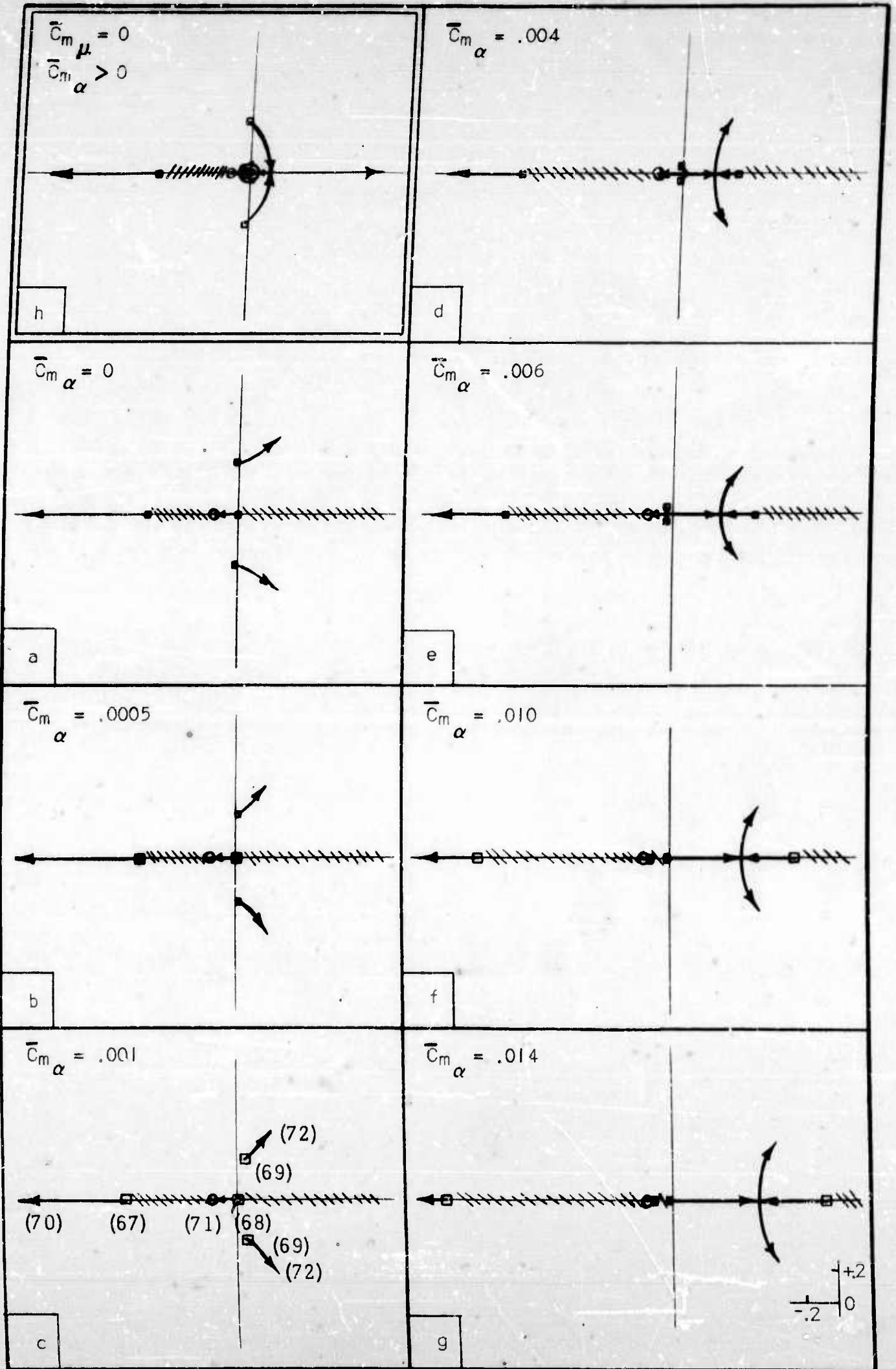
FIGURE 14 - I ROOT LOCUS S.C.D. \mu = 0.10 V = 36\text{MPH} \bar{C}_m \mu > 0
