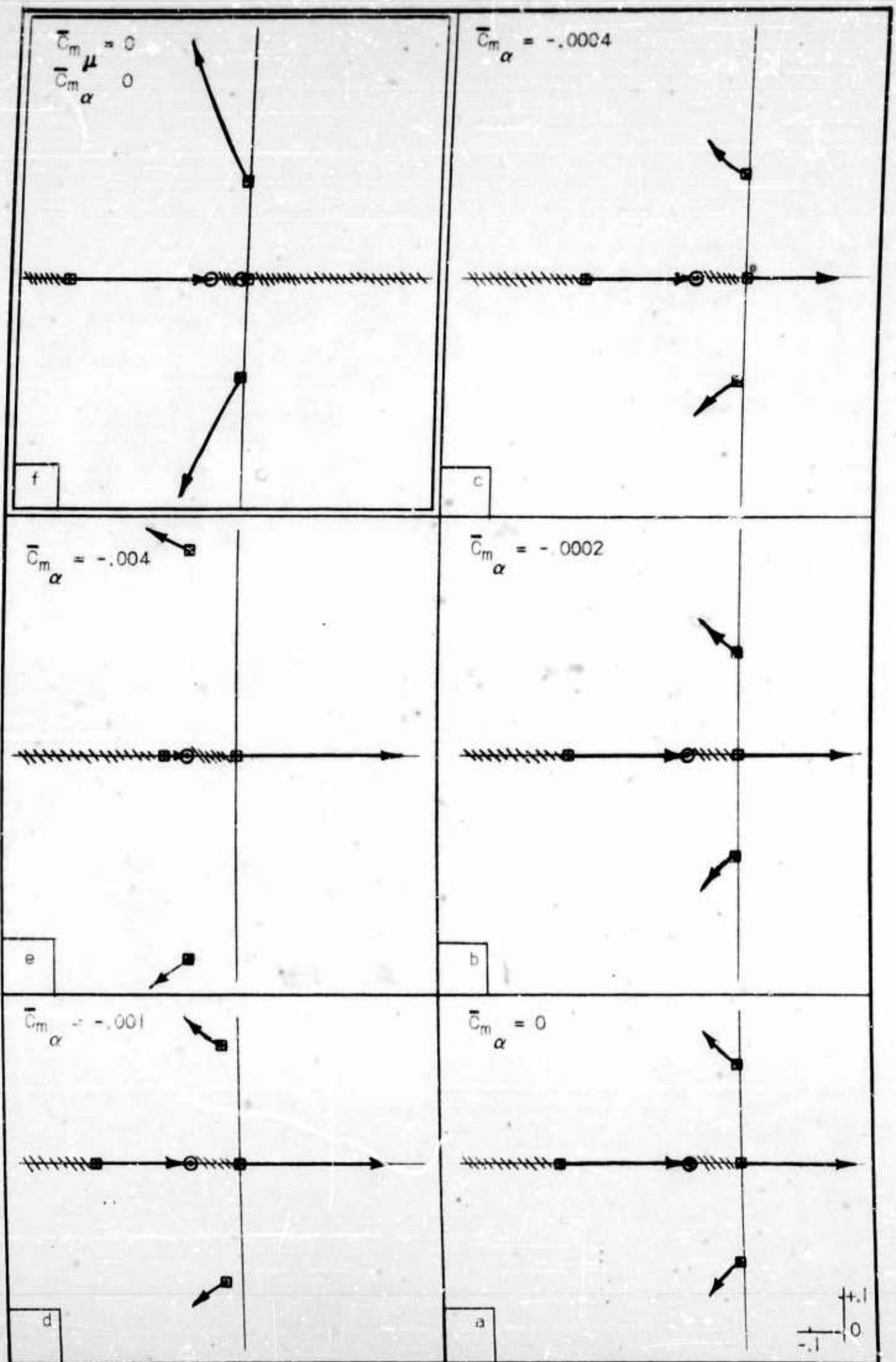
FIGURE 14 - III ROOT LOCUS S.C.D. \mu = 0.10 V = 35\text{MPH} \bar{C}_m < 0
