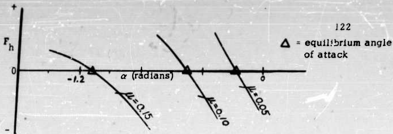
Fig. 21. Sketch of \alpha versus F_h for various \mu
