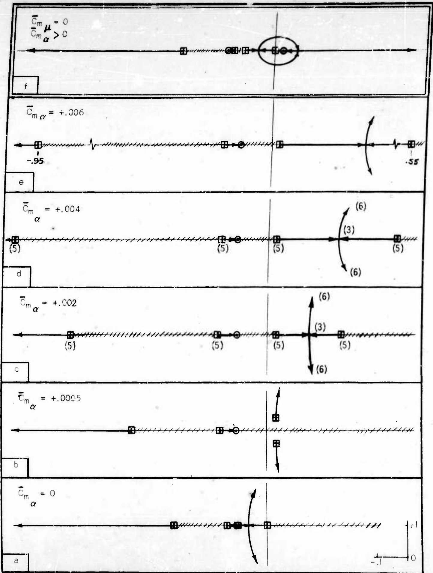
FIGURE 10 - I ROOT LOCUS L.C.D. \mu = 0.05 V = 16 MPH \bar{C}_m > 0
