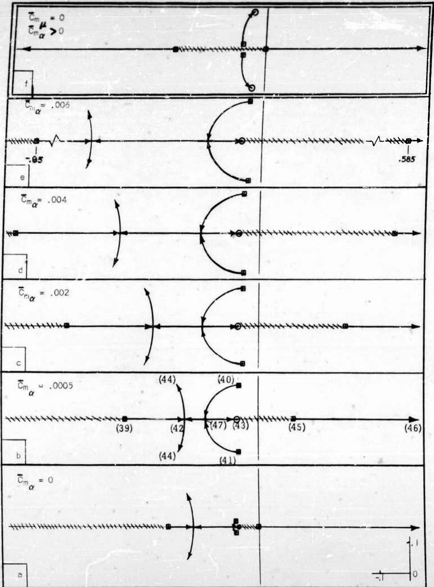
FIGURE 13 - IV ROOT LOCUS S.C.D.
