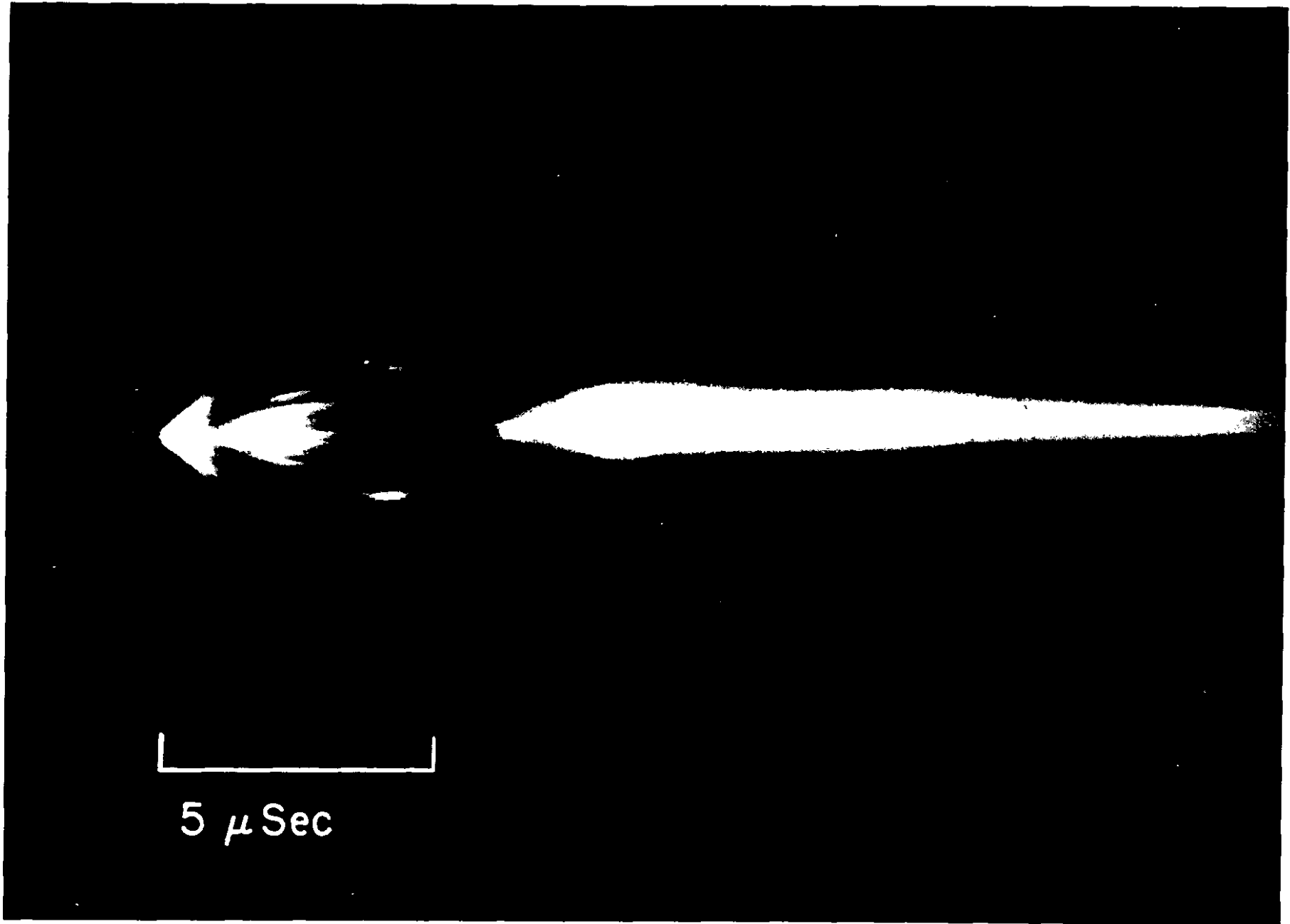
Fig. 2 Streak picture of 3.8 mil Cu wire at 8 kv.
