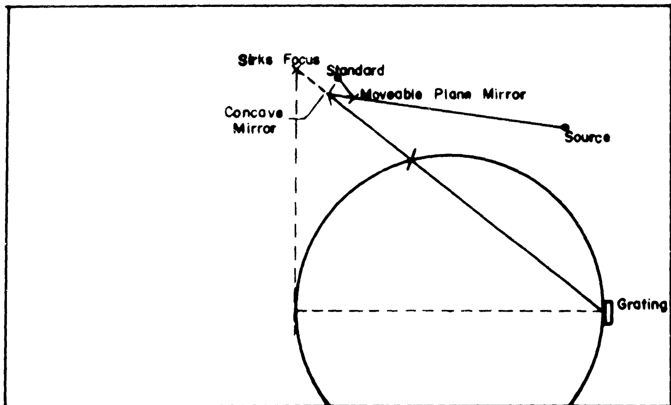
FIG 3a GRATING OPTICS
