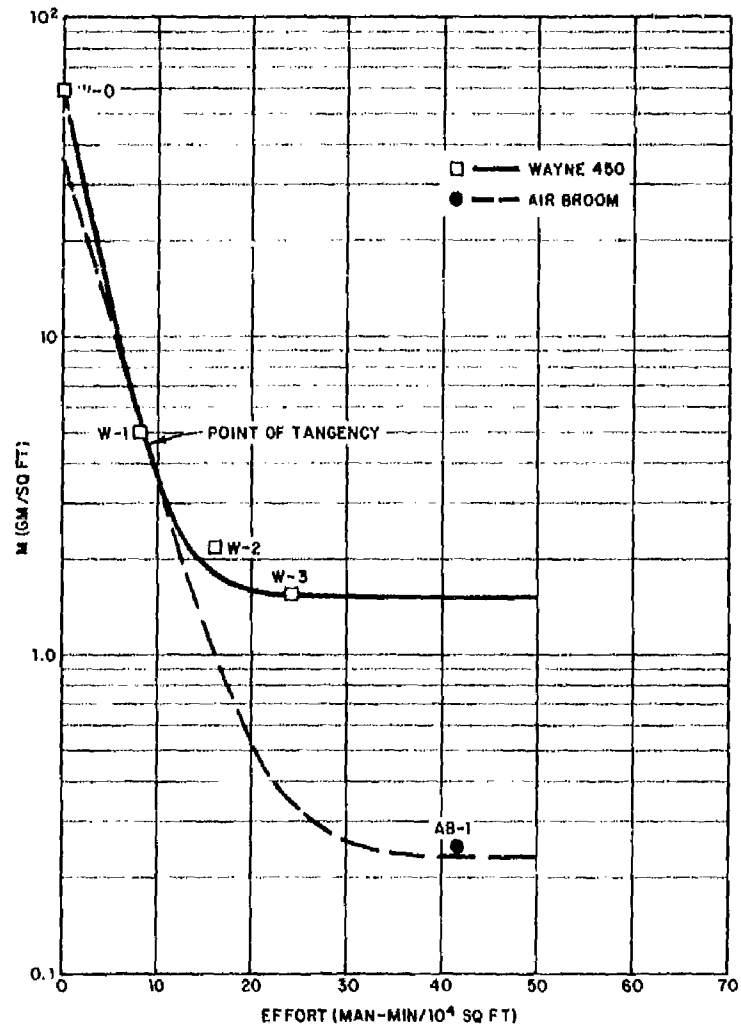
Fig. 4.3.2 Determination of the Path on Least Effort From Experimental Values for the Wayne 450 and the Air Broom (Test B-2):
