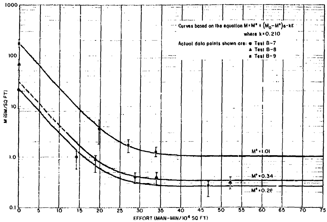
Fig. 4.1.4 Effectiveness of the Tennant 100 Vacuumized Sweeper on Asphaltic Concrete.
