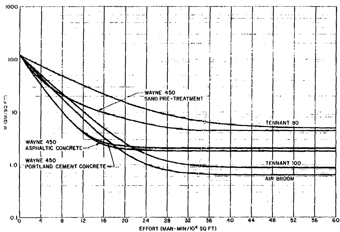
Fig. 4.2.3 Comparative Effectiveness of Dry Decontamination Methods on Paved Areas at an Initial Mass Level of 120 g/ft 2 .
