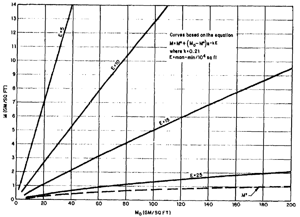
Fig. 4.4.3 Residual Mass vs Initial Mass - Tennant 100 Vacuumized Sweeping on Asphaltic Concrete.
