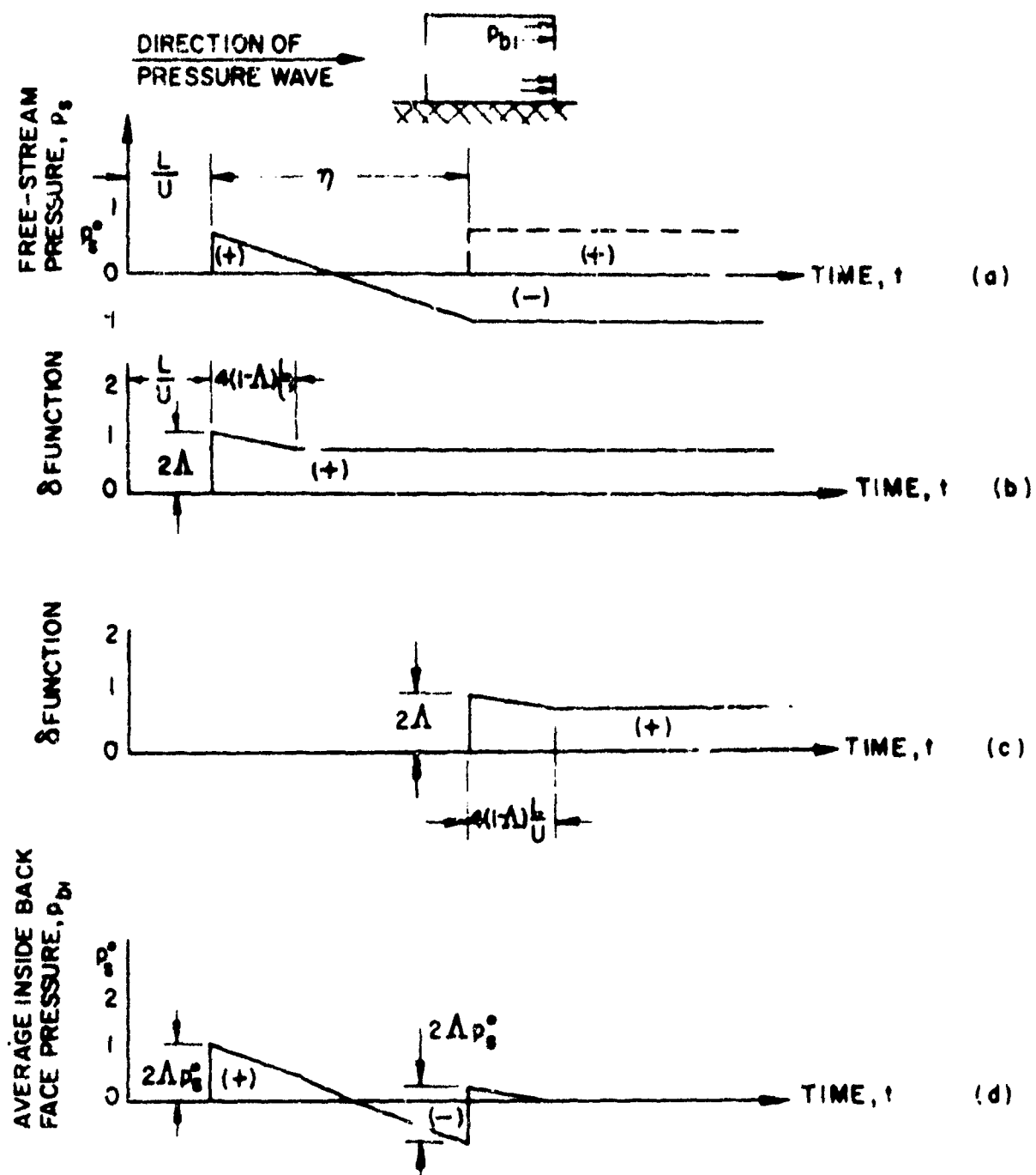
FIGURE 24 AVERAGE INSIDE BACK FACE PRESSURE PARTIALLY OPEN BUILDING- NORMAL INCIDENCE
