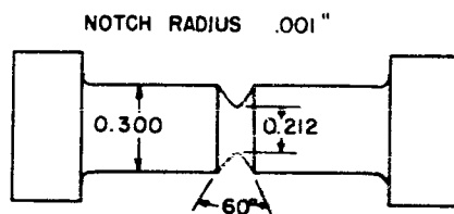
60° V NOTCH TENSILE SPECIMEN SPECIMEN TYPE B
