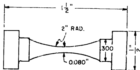
UNNOTCHED TENSILE SPECIMEN SPECIMEN TYPE A
