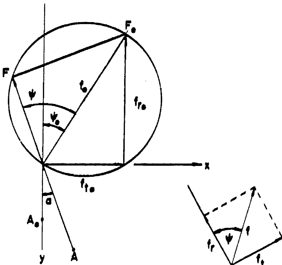
Fig. 32. Representation of resultant force.
