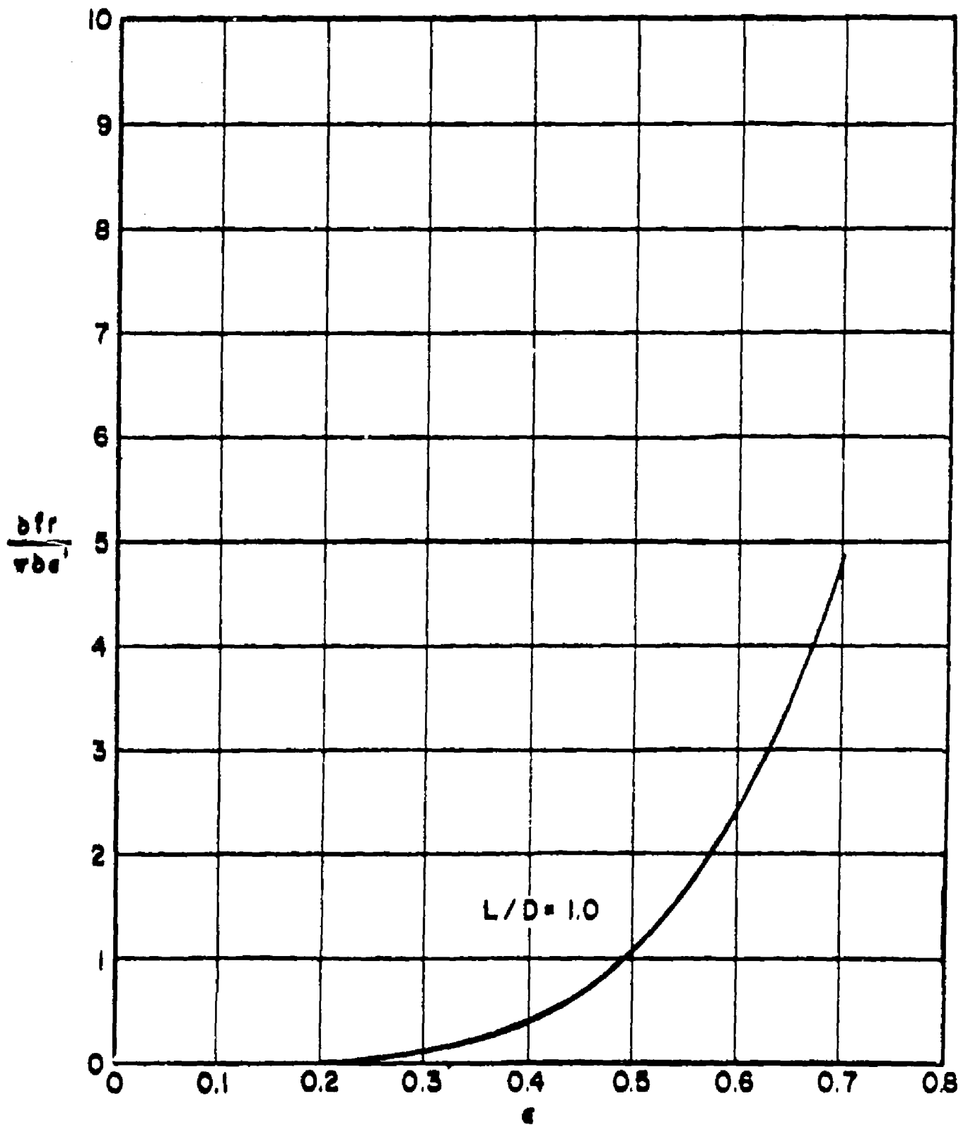
Fig. 23. \frac{\partial f_r}{\partial \epsilon} vs \epsilon (Compressible)
