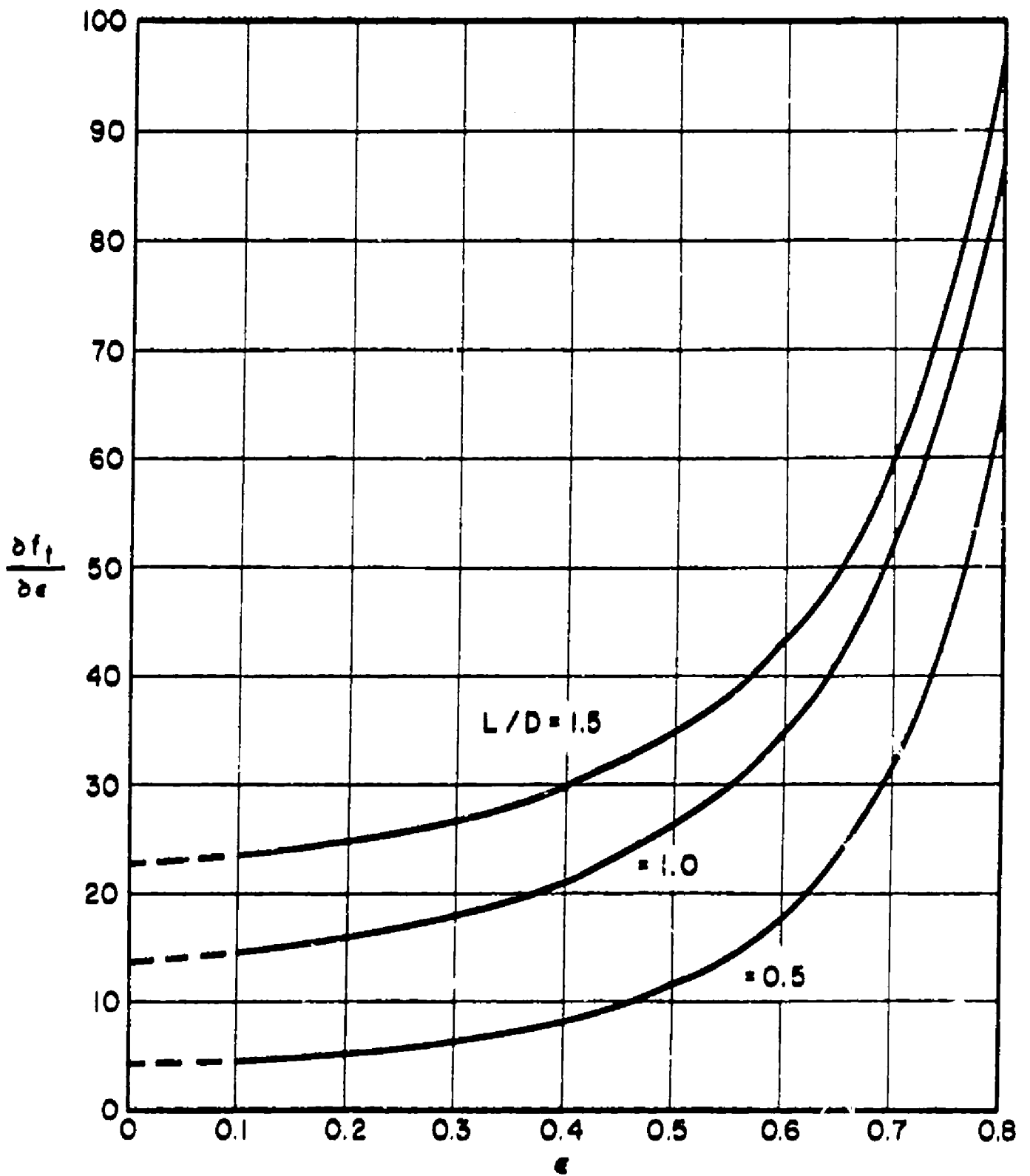
Fig. 24. \frac{\partial f_1}{\partial \epsilon} vs \epsilon (Compressible)
