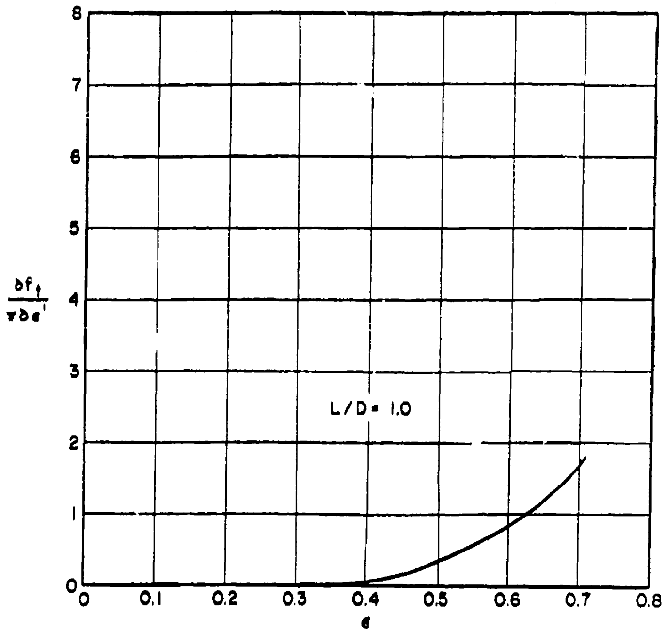
Fig. 25. \frac{\partial f_t}{\pi \partial \alpha} vs \alpha (Compressible)
