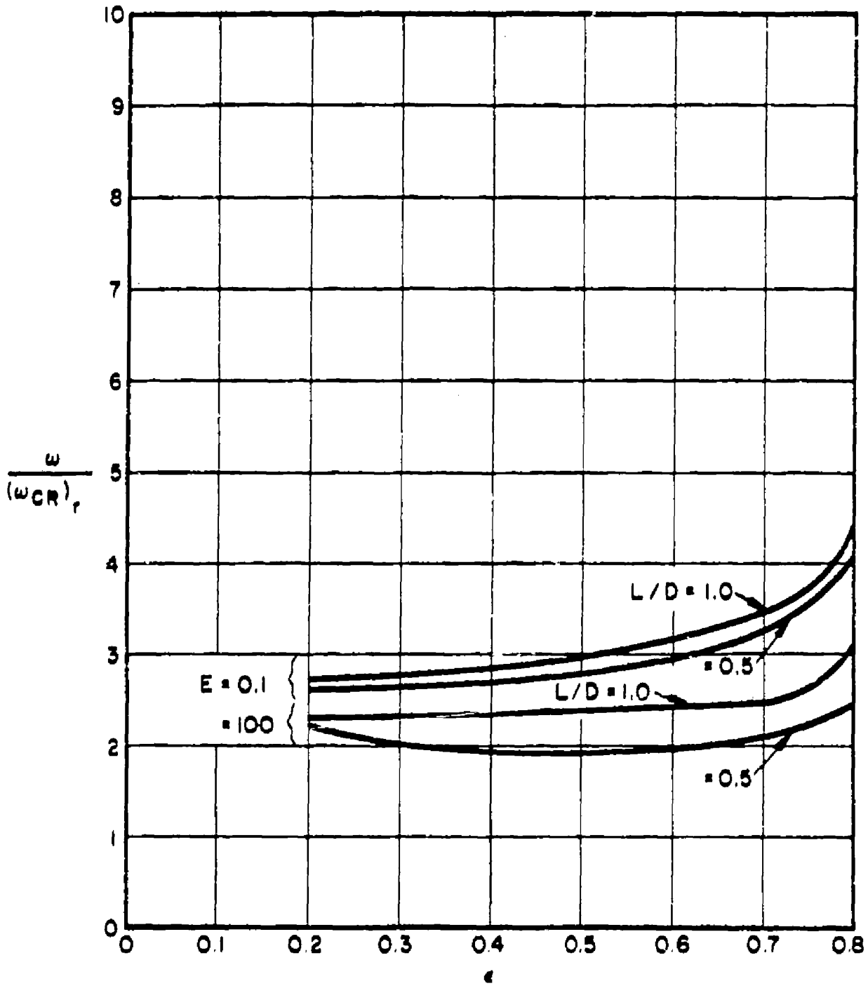
Fig. 28. (\omega/\omega_{CR})_r vs \epsilon for incompressible cases.
