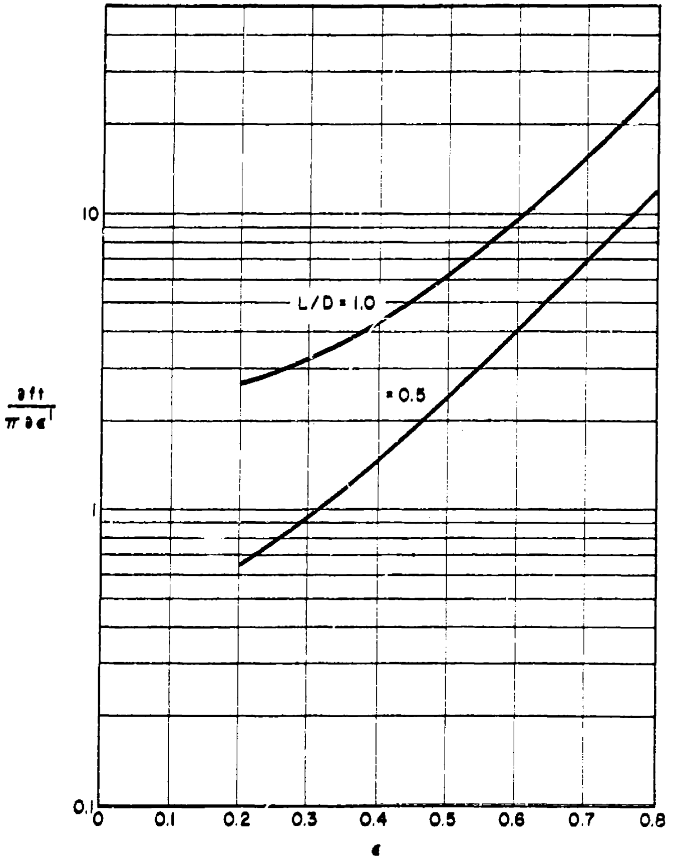
Fig. 21. \frac{\partial f_t}{\pi \partial \alpha} vs \alpha (incompressible).
