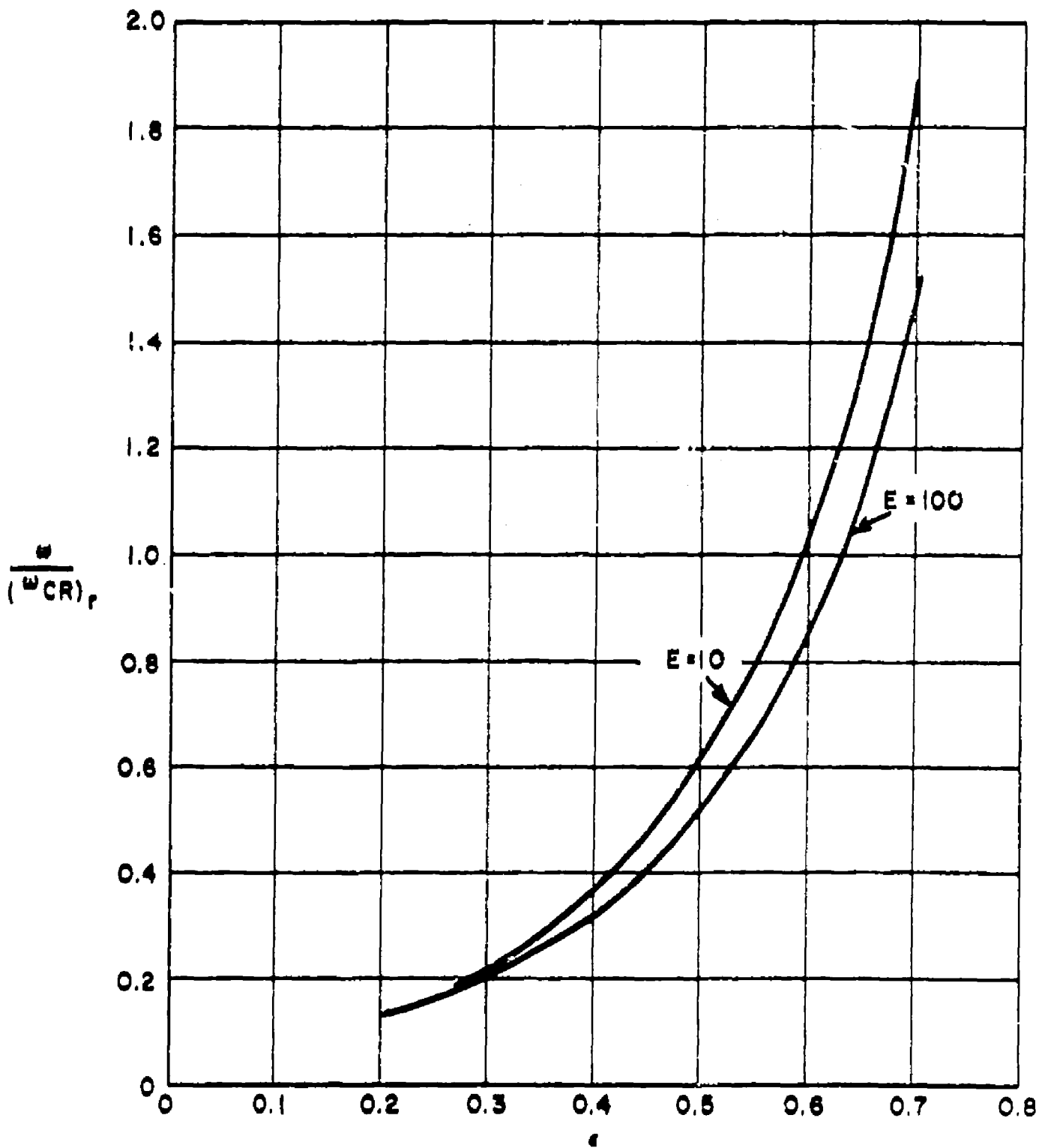
Fig. 30. \frac{\omega}{(\omega_{CR})_r} vs e for compressible cases.
