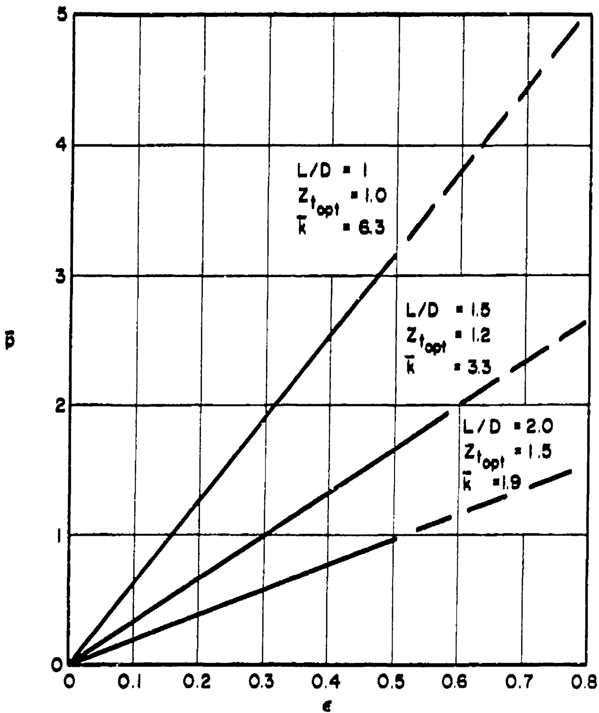
Fig. 10. Dimensionless pressure vs eccentricity ratio P_5/P_a = 12 .
