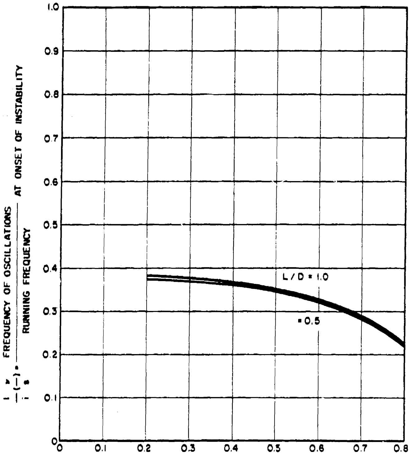
Fig. 29. \frac{1}{\epsilon} \left( \frac{Y}{S} \right) vs \epsilon for incompressible cases.
