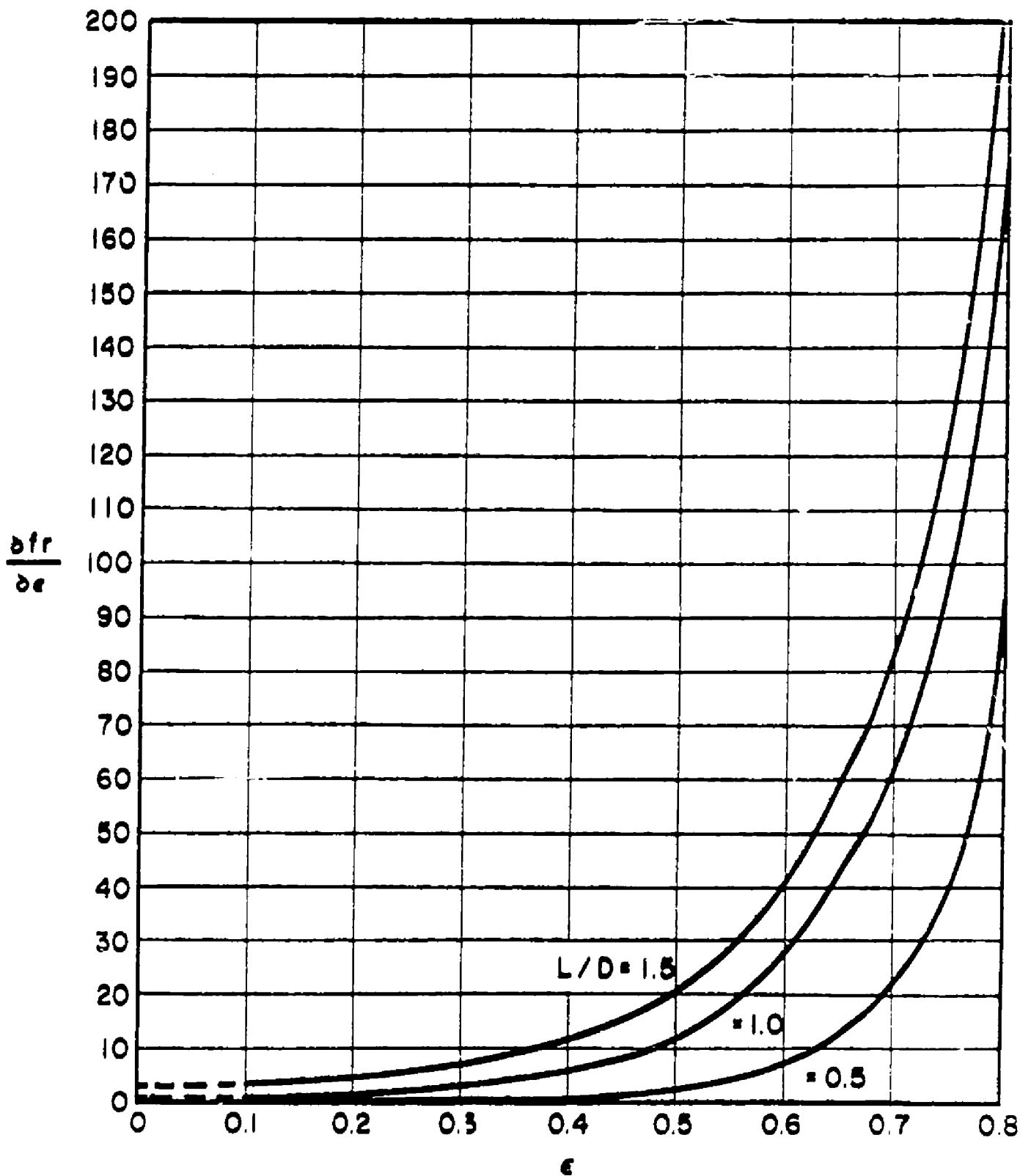
Fig. 22. \frac{\partial r}{\partial \epsilon} vs \epsilon (Compressible)
