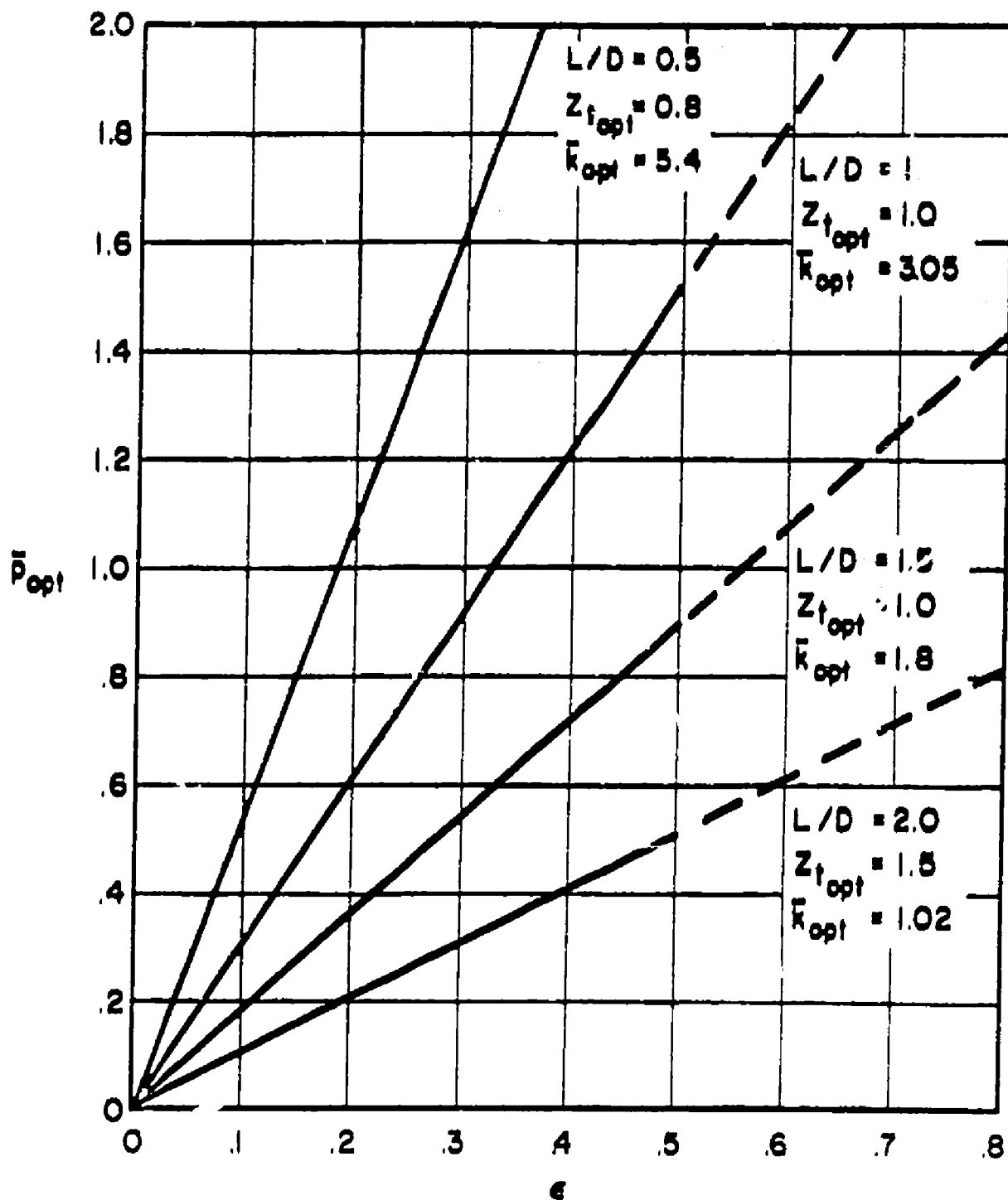
Fig. 9. Dimensionless pressure vs eccentricity ratio P_S/P_B = 6 .
