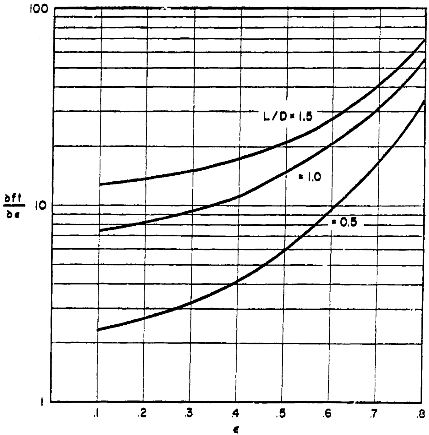
Fig. 20. \frac{\partial f_t}{\partial \epsilon} vs \epsilon (Incompressible)
