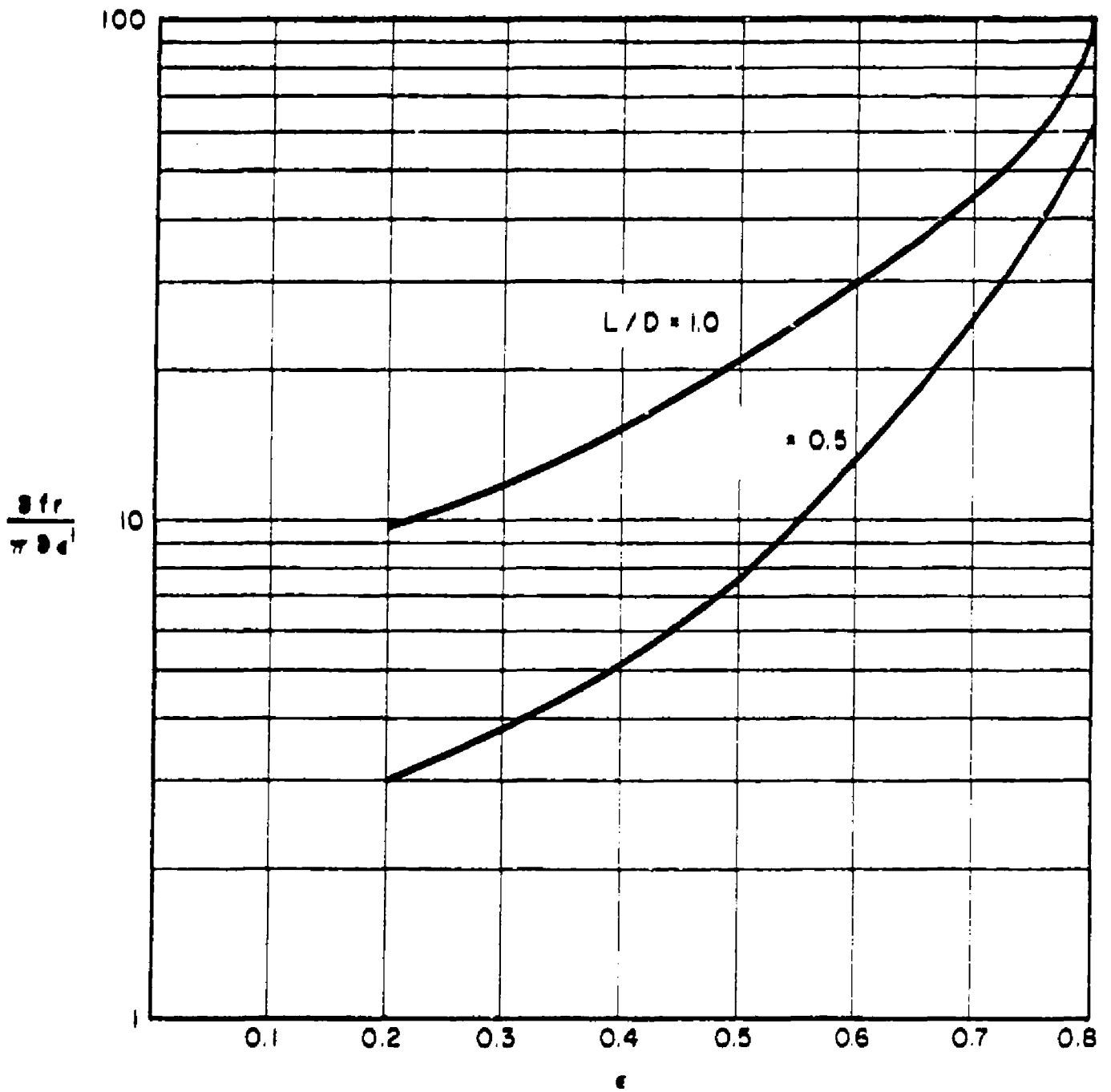
Fig. 19. \frac{8f_r}{\pi D_e^3} vs \epsilon (incompressible).
