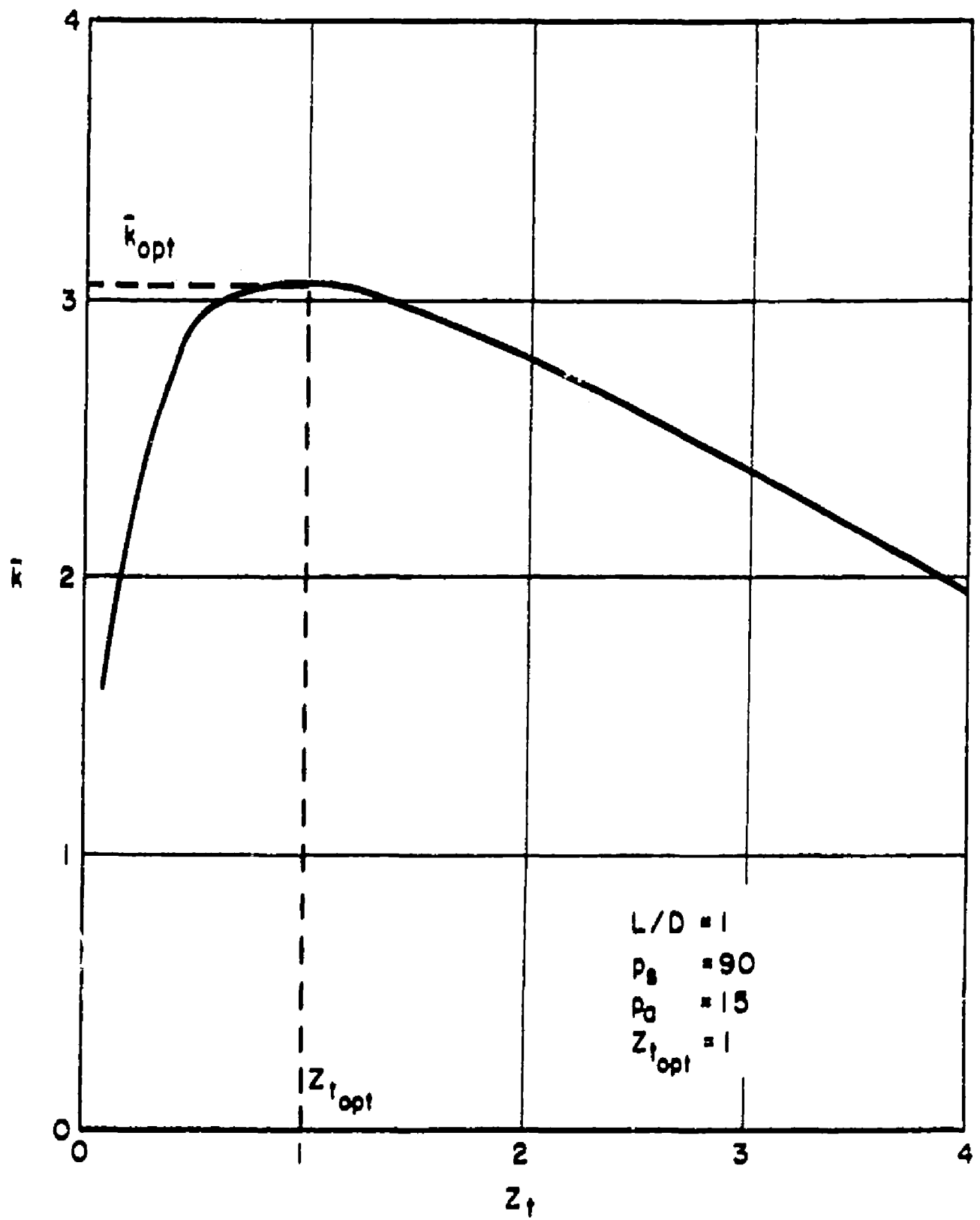
Fig. 7. Dimensionless feeding parameter Z_t vs dimensionless stiffness \bar{k} .
