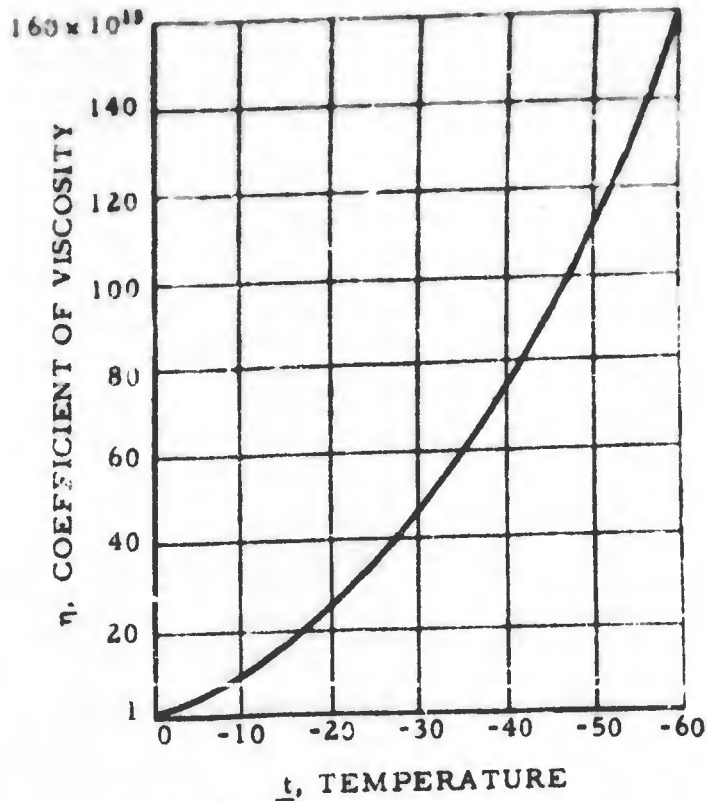
Figure 3. Relationship between coefficient of viscosity of ice and temperature.
