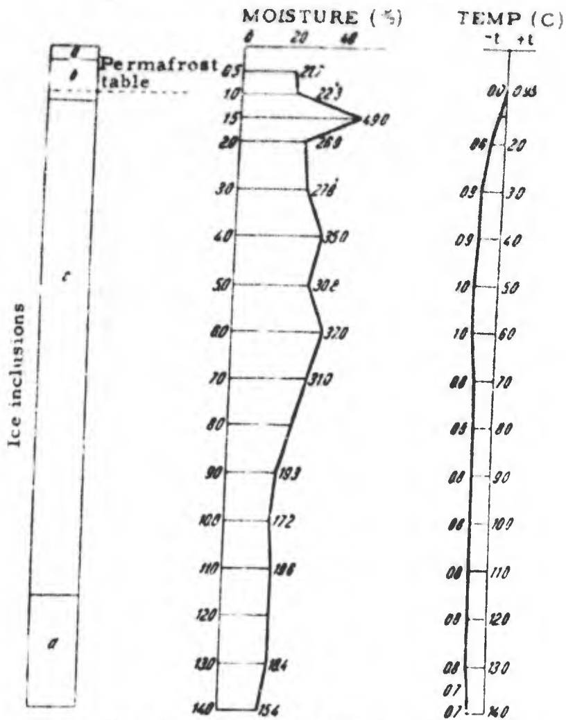
Figure 118. Cross section 3.
