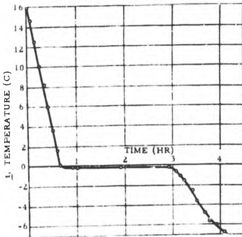
Figure 6. Ground temperature vs time.
