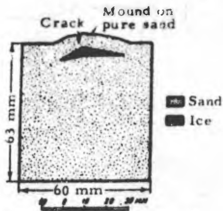
Figure 16. Formation of ice lens in sand.
