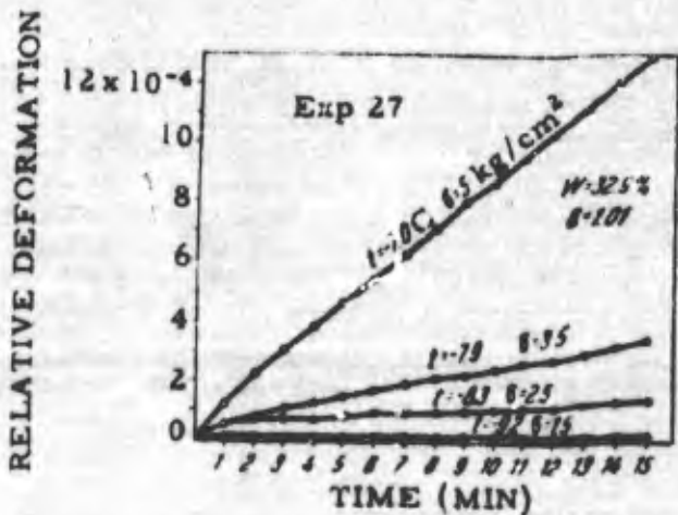
Figure 69. Relative deformation of frozen clay under constant load.
