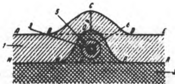
Figure 104. Third variant of water pipe placement. Pipe is laid at a certain depth in the active layer. 1) Active layer; 2) Permafrost; 3) Water pipe; 4) Moisture - bearing soil; 5) Insulating layer (peat).
