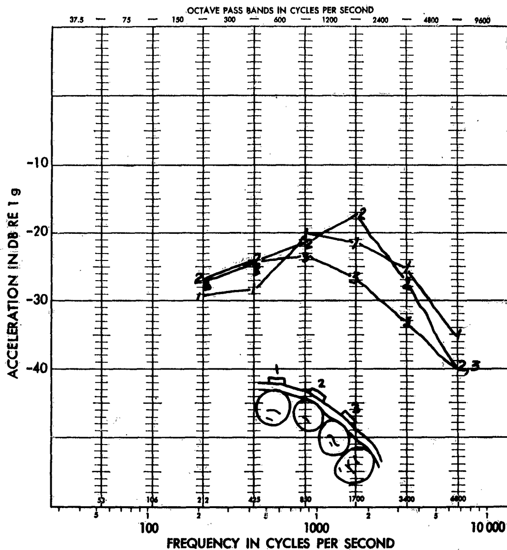
EFFECT OF ACCELEROMETER POSITION ON TOOTH VENEER ON SPEECH PICKUP Subject: JPC
