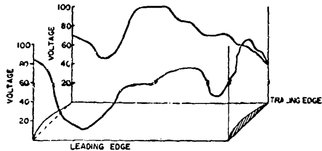
Fig. 2 - Voltage distribution on port-wing edges of an AD-6 aircraft
