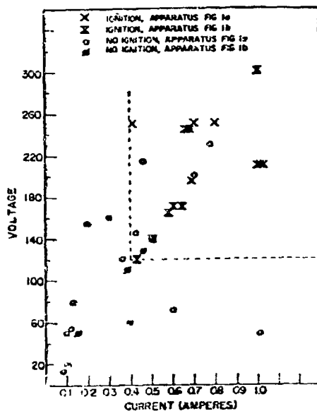
Fig. 4 - Ignition studies at various arc voltages and currents
