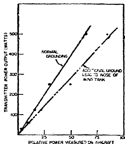
Fig. 3 - Transmitter output vs relative power measured on aircraft
