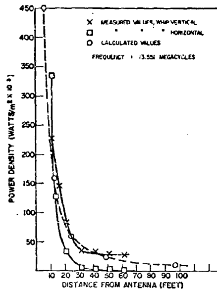
Fig. 5 - Field intensity vs distance from antenna
