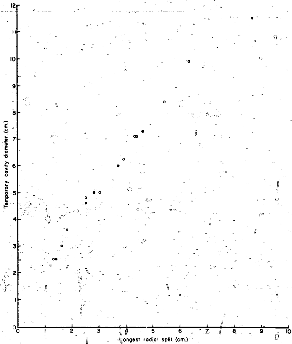
FIGURE 4 TEMPORARY-CAVITY DIAMETER VS. LONGEST RADIAL SPLIT IN 20% GELATIN.
