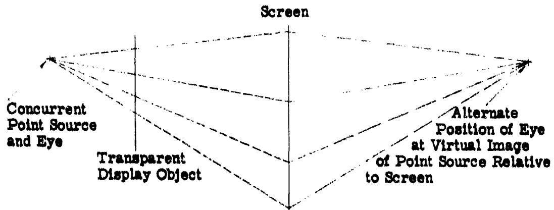
a. Projection of Transparent Display Object
