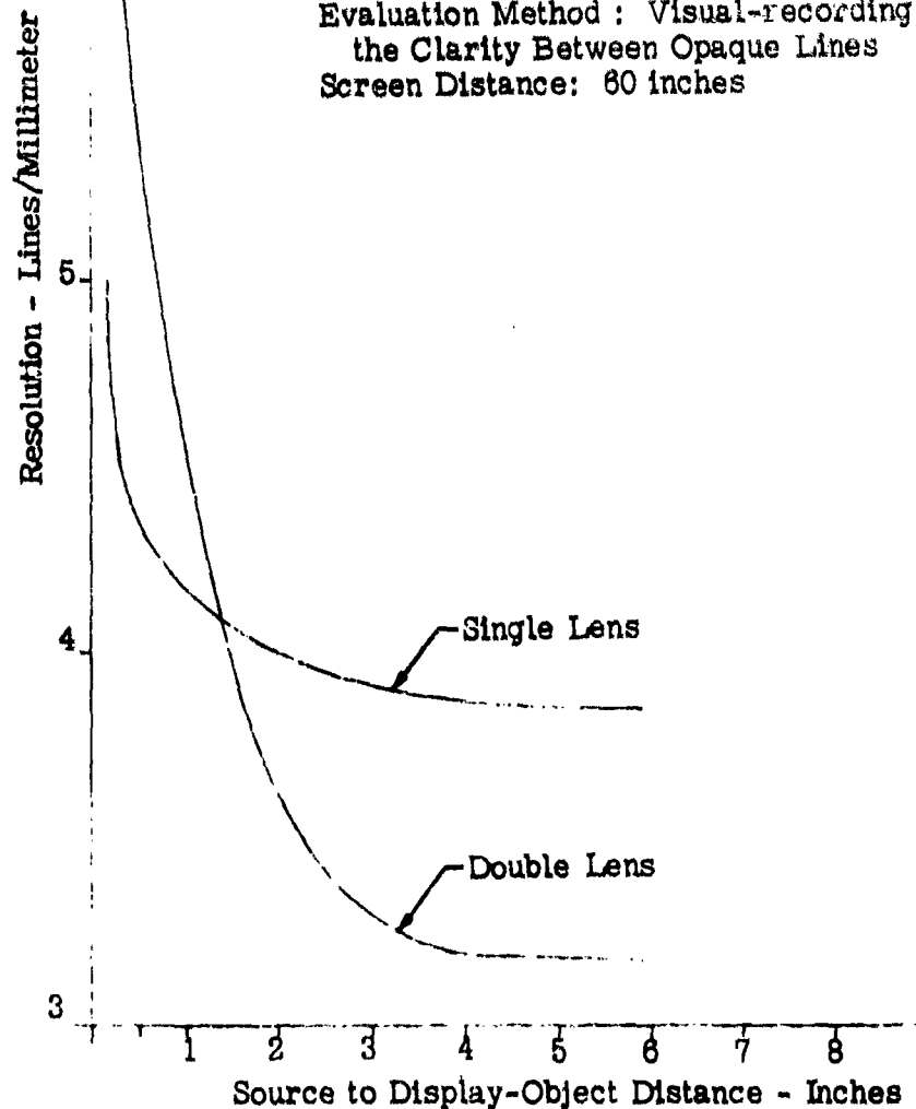
Figure V - 6 - Effect of Source to Display-Object Distance on Resolution for Single and Double Meniscus Lens Systems.
