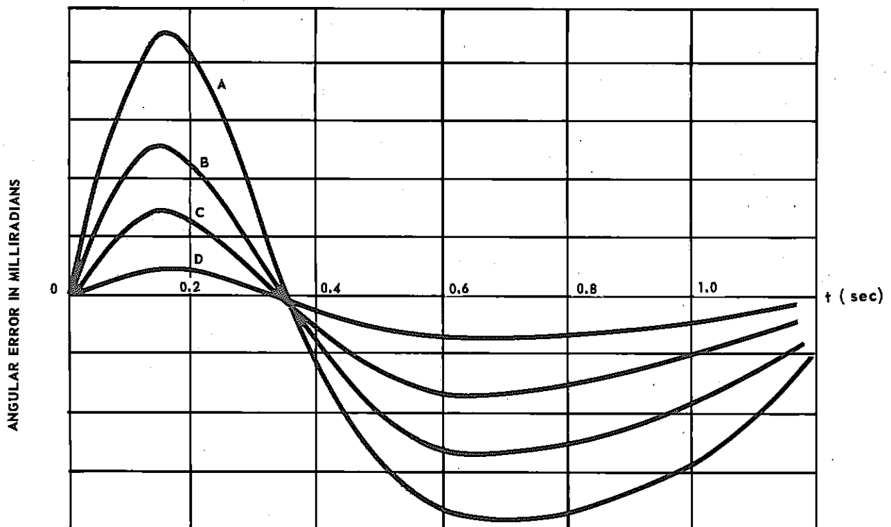
FIGURE 8-18. ANGULAR ERROR DUE TO ROLL TRANSIENT AS A FUNCTION OF STABILIZATION BANDWIDTH
