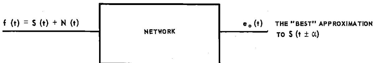
FIGURE G-1. WIENER PROBLEM
