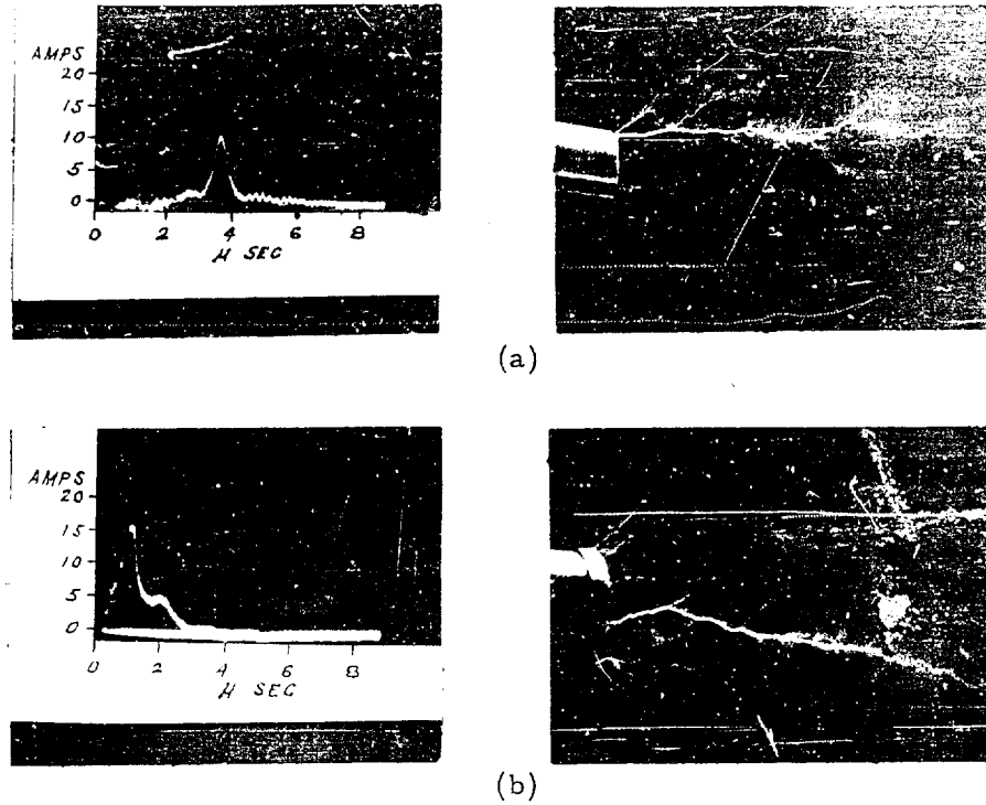
Figure 6. Current waveforms and photographs of single streamers.
