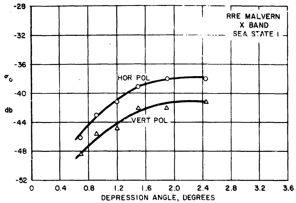
FIG. 2-10 RRE Sea clutter measurements for horizontal and vertical polarisations
