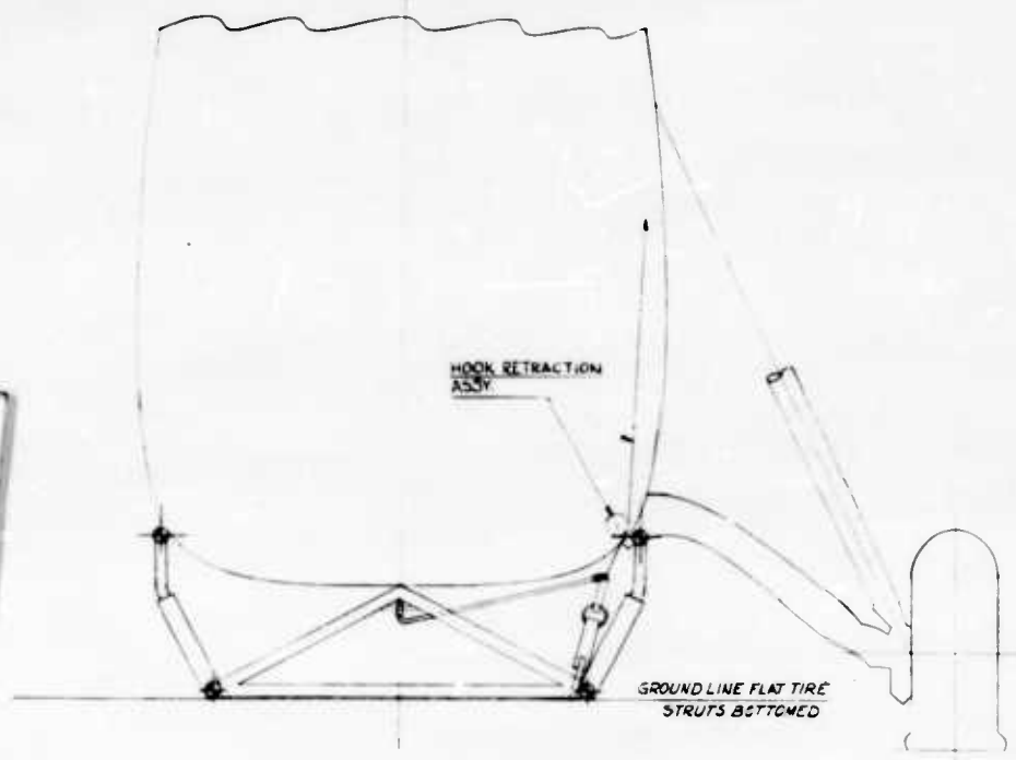
VIEW LOOKING AFT CARGO SWING RETRACTED
