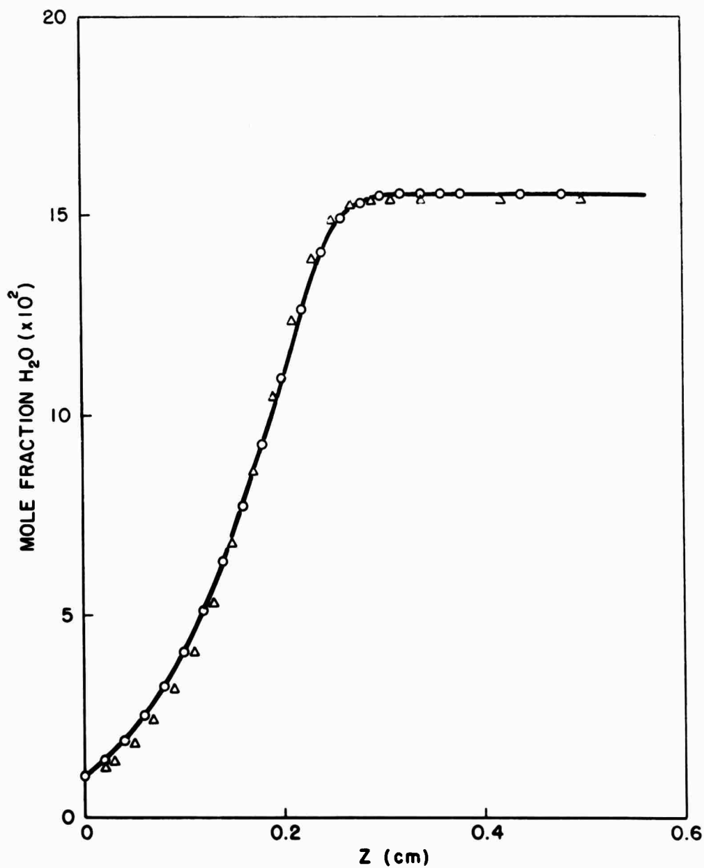
Fig. 1-2 PLOT SHOWING CONGRUENCE OF THE WATER MOLE FRACTION PROFILE IN THE \text{CH}_4\text{-O}_2 FLAME AT TWO PRESSURES
