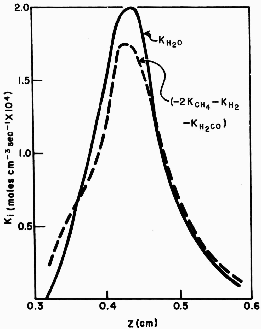
Fig. I-4 COMPARISON OF K_{H_2O} WITH THE COMBINED RATE (-2K_{CH_4} - K_{H_2} - K_{H_2CO}) Pressure = 1/20 atm.
