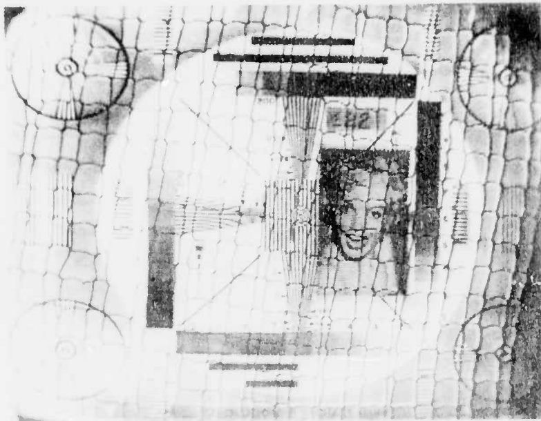
Figure 10 - This photograph shows a monitor view of tube #122 which has a piece of dynoid mesh used as a target mesh with a P-8 spacing of .010". It illustrates the imaging quality of such a tube and points out the visibility of large (.002") wire when used for target mesh.
