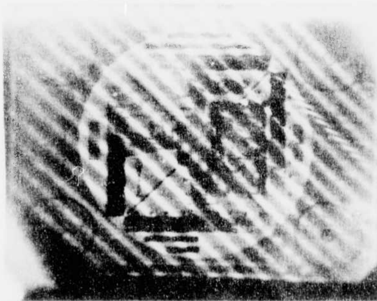
Figure 12- Stretched wire grid tube #155 showing appearance of image when the tube is subject to impact. Note the different frequency and intensity of the vibration of various wires. These wires were mounted with varying tensions.
