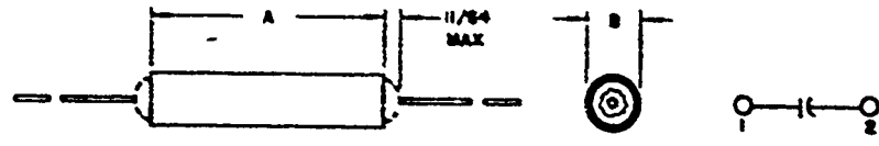
Figure 1 - Dimensions and Circuit Diagram
