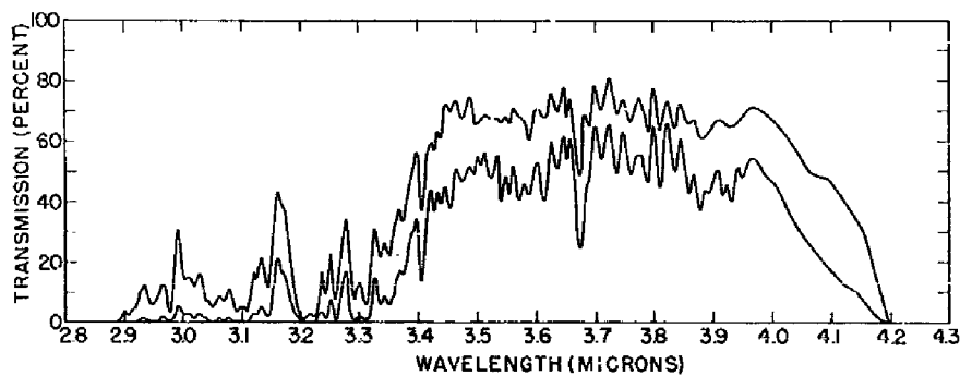
Fig. 5 - Atmospheric transmission over 5.5 km and 16.25 km in the Chesapeake Bay area. Data from runs 58 and 60 over 5.5 km and from runs 59 and 61 over 16.25 km.
