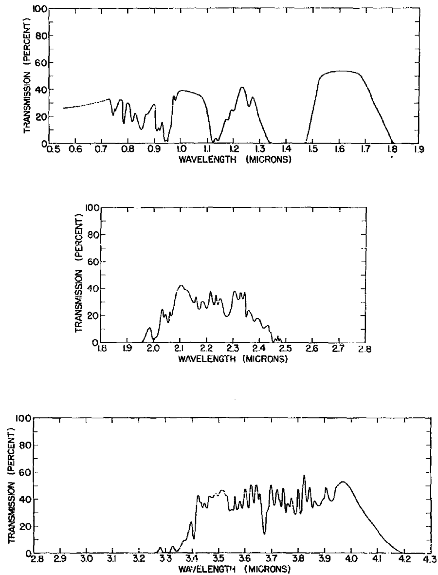
Fig. 9 - Atmospheric transmission over 27.7 km in the Hawaiian Islands. Data from run ML-3.
