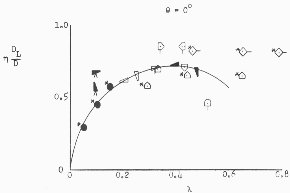
FIGURE 3: COMPARISON OF PROPULSIVE EFFICIENCIES FOR DIFFUSED AND NON-DIFFUSED DUCTED PROPELLERS IN AXIAL FLOW
