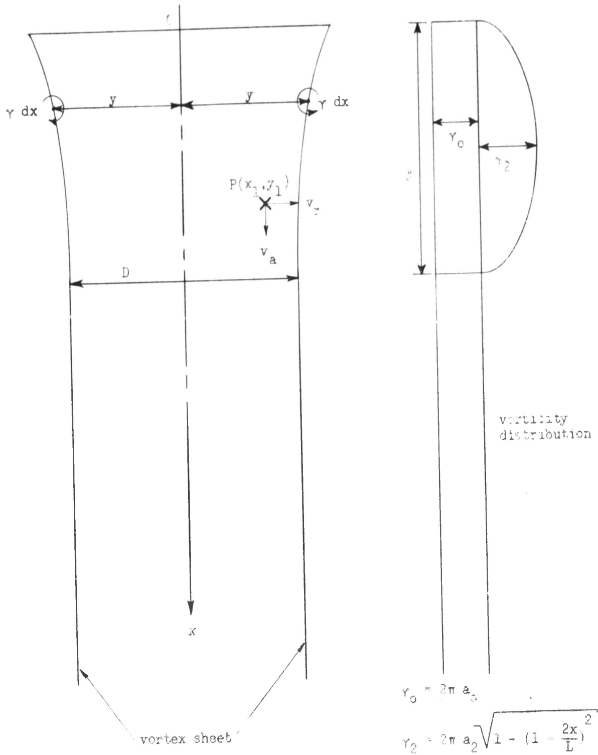
FIGURE 23: MATHEMATICAL MODEL FOR DUCT SHAPE AND VORTICITY DISTRIBUTION
