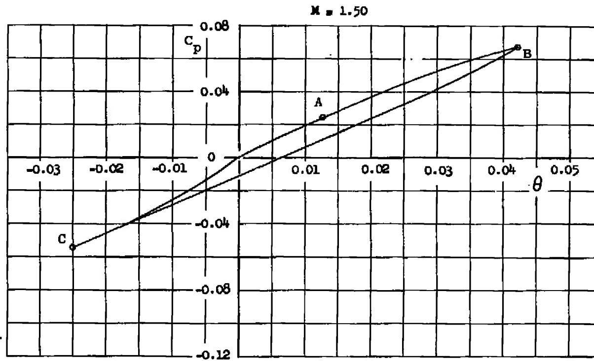
Fig. 1 Required Flow Characteristics in the Flow Field about a 20^\circ Cone-Cylinder Model of 2-Percent Blockage at a Position Corresponding to the Tunnel Wall
