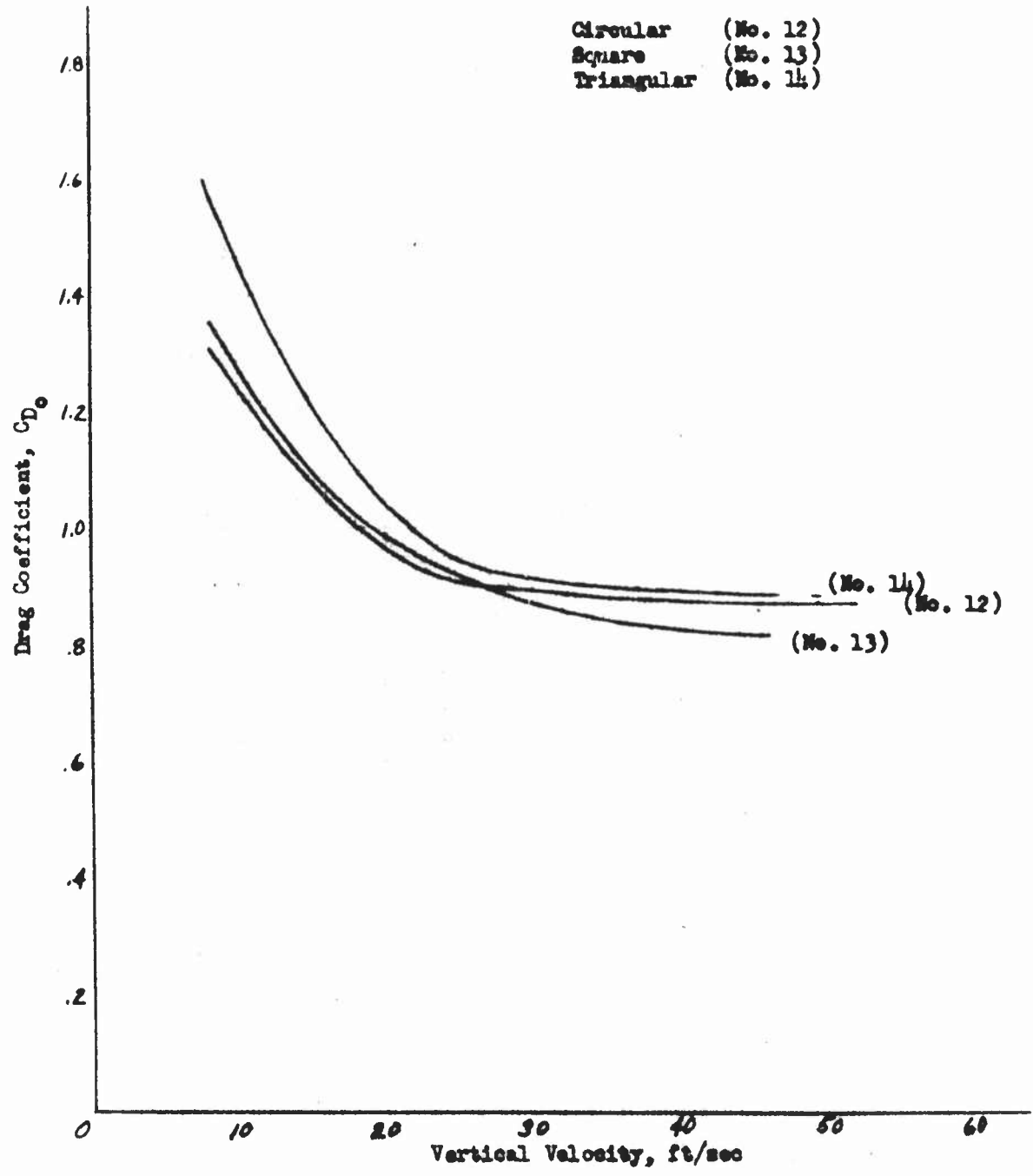
Figure 73 - Summary curves of drag coefficient versus vertical velocity for the models of the 30° solid conical parachute family
