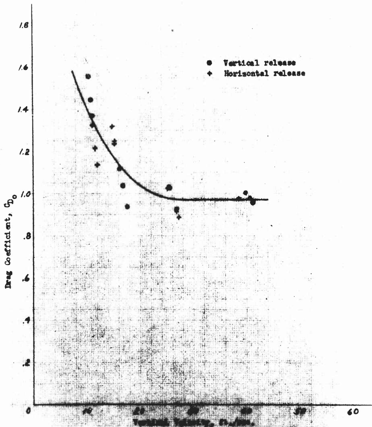
Figure 53- Drag coefficient versus vertical velocity for the solid-flat-convex paraboloid (No. 1) measured during free fall after both vertical and horizontal types of release.
