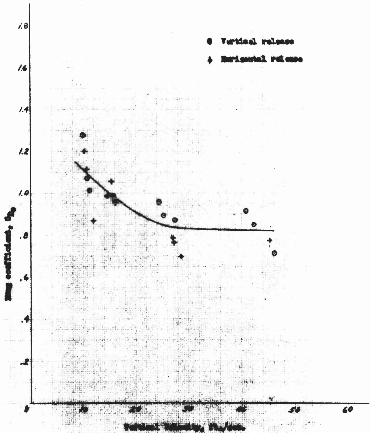
Figure 25 - Drag coefficient vs. velocity for the solid- rocket motor (No. 2) measured for vertical and horizontal types
