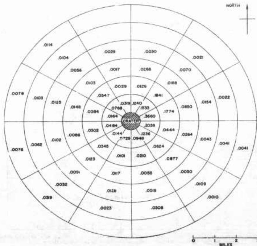
FIGURE 6.—Average percentages of size 40 meteoritic material in the soil around the crater.
