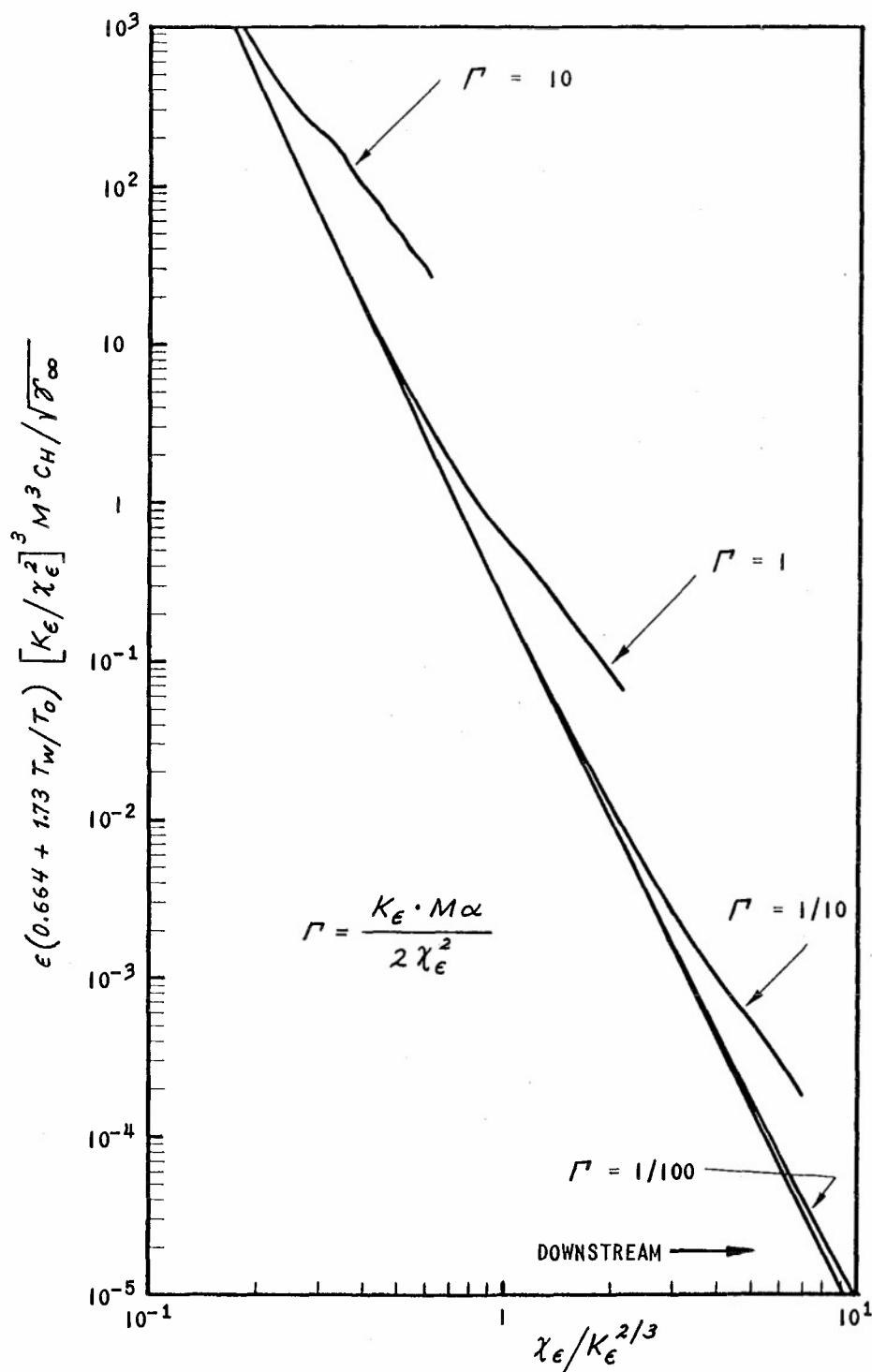
(a) SURFACE HEAT-TRANSFER RATE
