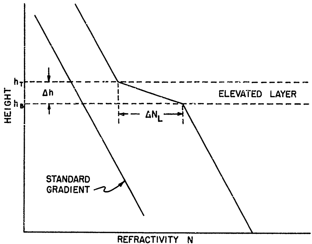
Figure 5.1. N-Profile--Elevated Layer.
