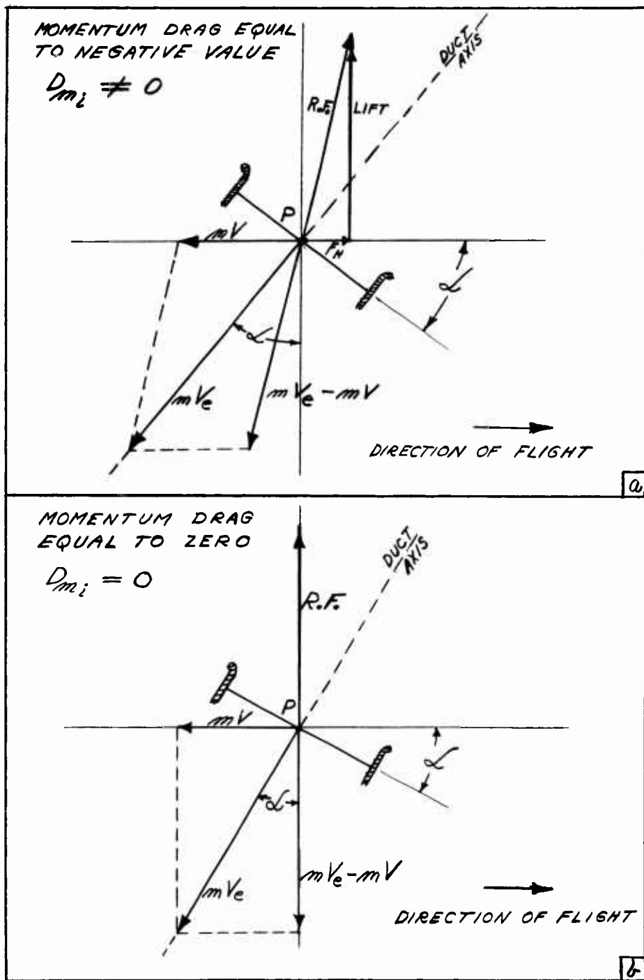
FIG. 2 VECTOR DIAGRAM FOR SINGLE DUCT
