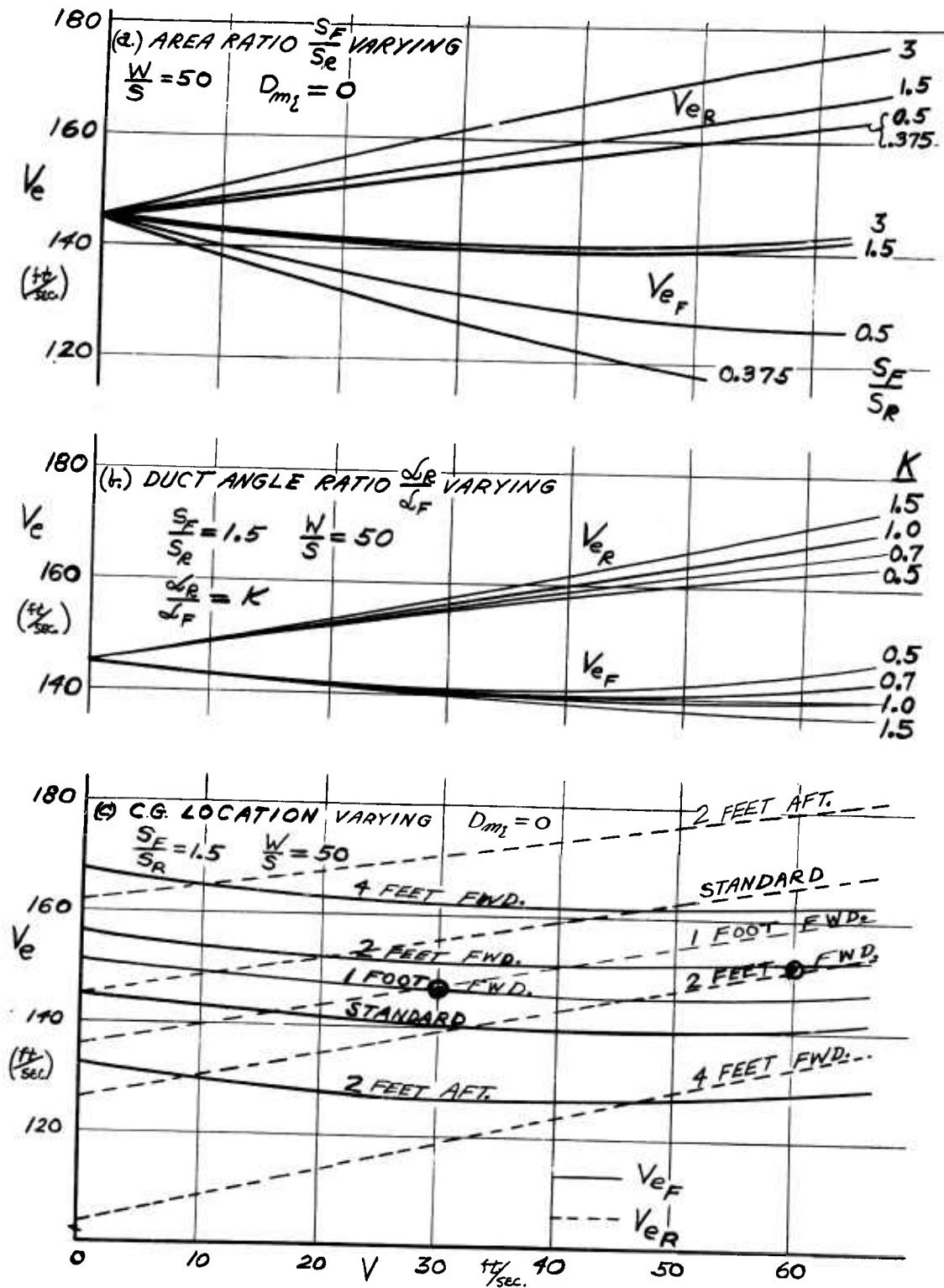
FIG. 7 DUCT EXIT VELOCITY vs. FORWARD SPEED
