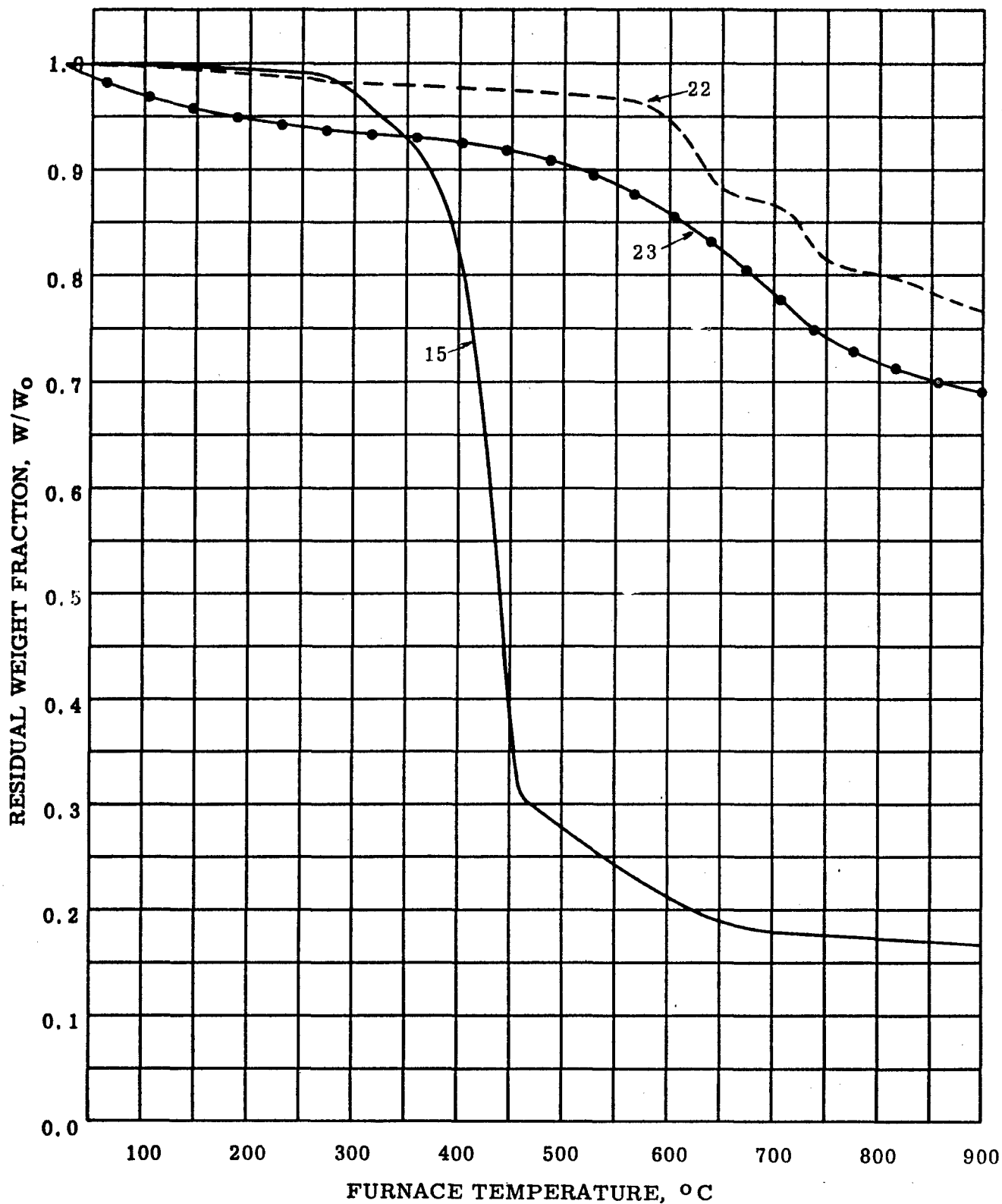
Figure 16 TGA IN DRY N 2 AT 180 C° PER HOUR COPPER PHTHALOCYANINE POLYMERS
