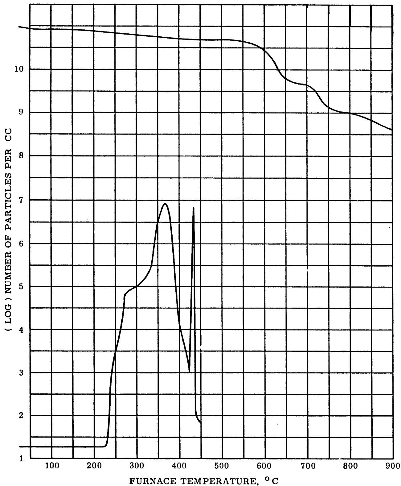
Figure 56 TPA IN DRY N_2 AT 180\text{ C}^\circ PER HOUR, COMPARED WITH TGA AT THE SAME HEATING RATE, COPPER PHTHALOCYANINE ( MATERIAL 22 )
