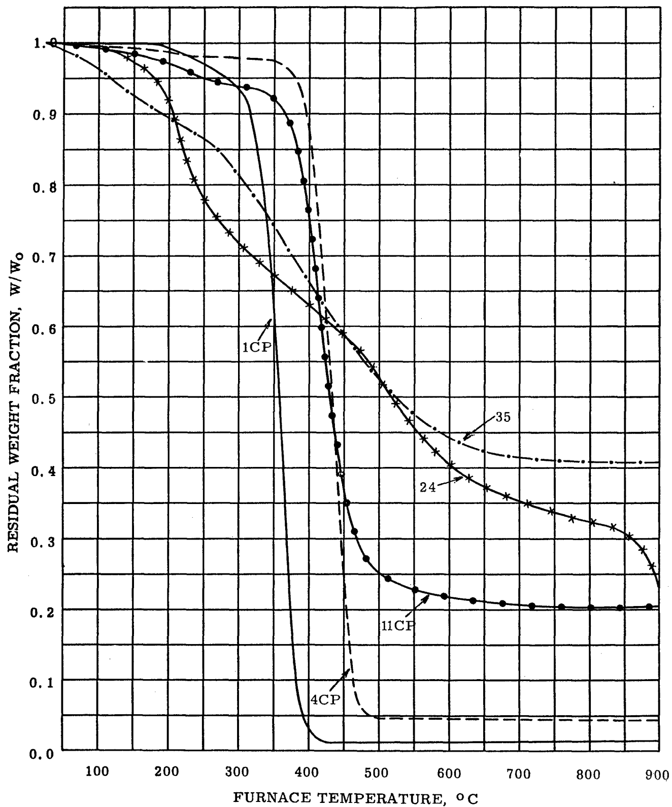
Figure 10 TGA IN DRY N 2 AT 180 C° PER HOUR
