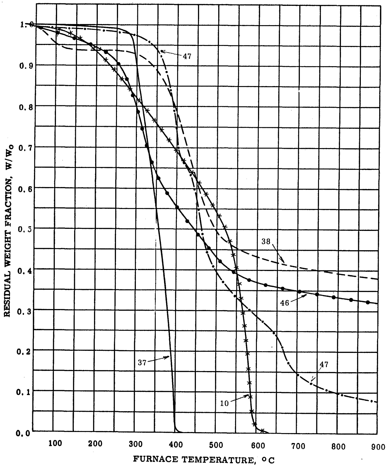
Figure 11 TGA IN DRY N_2 AT 180^\circ C PER HOUR TRIAZINE RING AND ISOCYANATE POLYMERS
