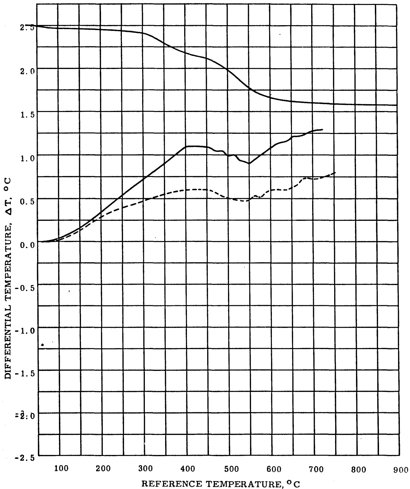
Figure 46 DTA IN DRY N_2 AT 180\text{ }^\circ\text{C} PER HOUR, COMPARED WITH TGA AT THE SAME HEATING RATE, RESIN OF Me_2N + Me_2P + B + H (BURG)
