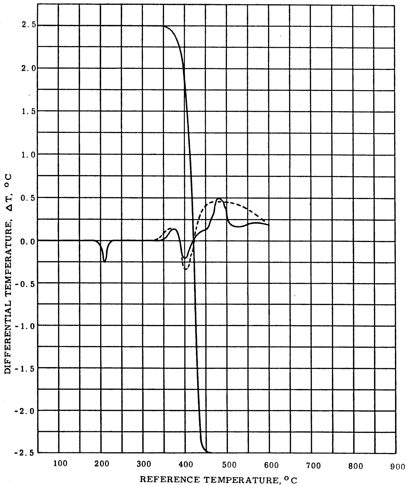
Figure 44 DTA IN DRY N_2 AT 180 C° PER HOUR, COMPARED WITH TGA AT THE SAME HEATING RATE, POLYCHLOROTRIFLUOROETHYLENE
