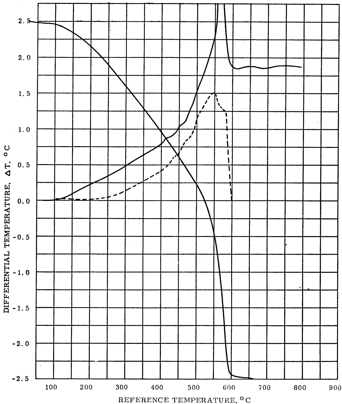
Figure 45 DTA IN DRY N 2 AT 180 C° PER HOUR, COMPARED WITH TGA AT THE SAME HEATING RATE, PERFLUOROGLUTARODIAMIDINE-PERFLUOROBUTYRAMIDINE COPOLYMER, CODE 282
