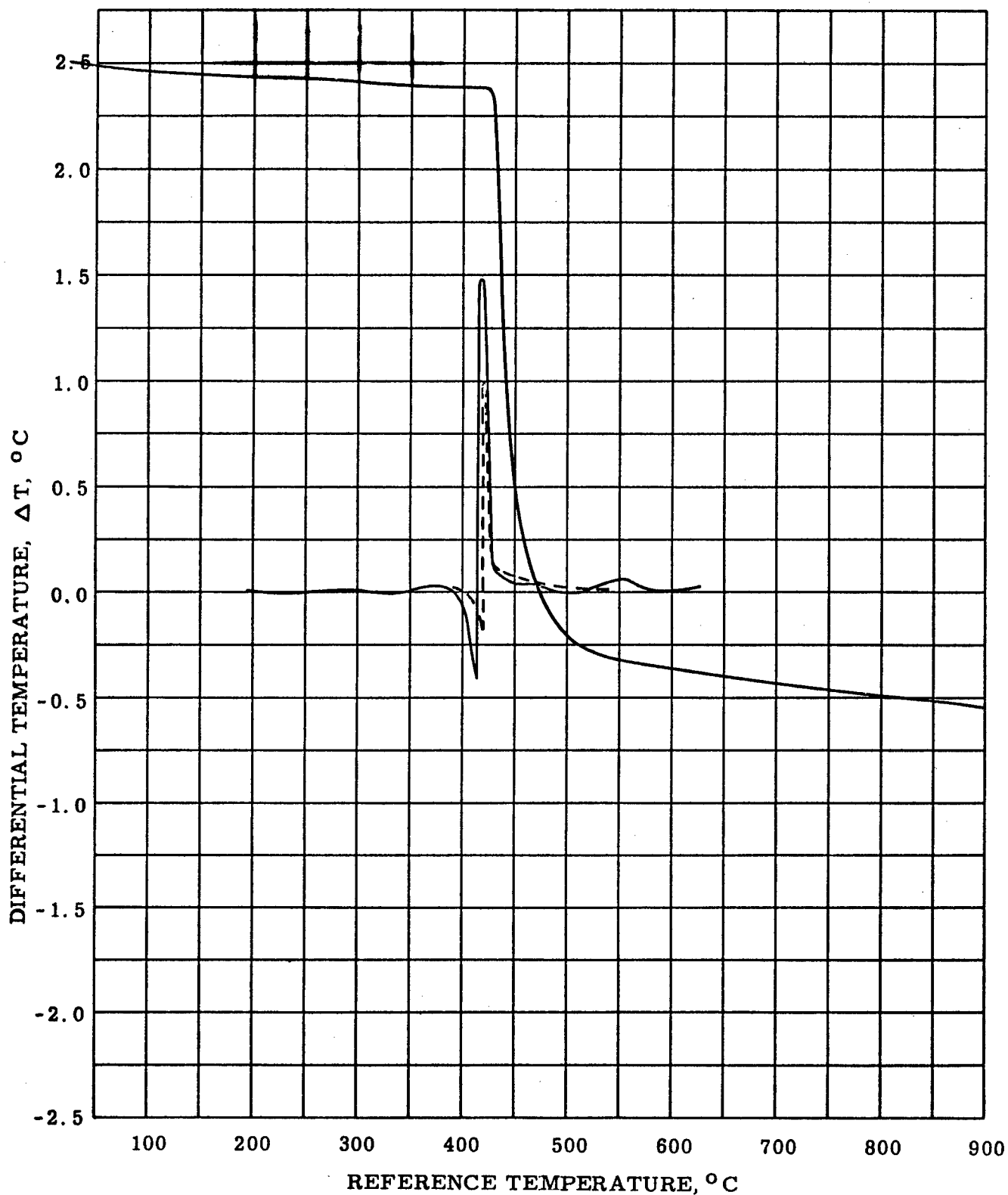
Figure 49 DTA IN DRY N_2 AT 180\text{ }^\circ\text{C} PER HOUR, COMPARED WITH TGA AT THE SAME HEATING RATE, ZINC 4, 4' - BIS - THIOPICOLINAMIDODIPHENYL SULFONE
