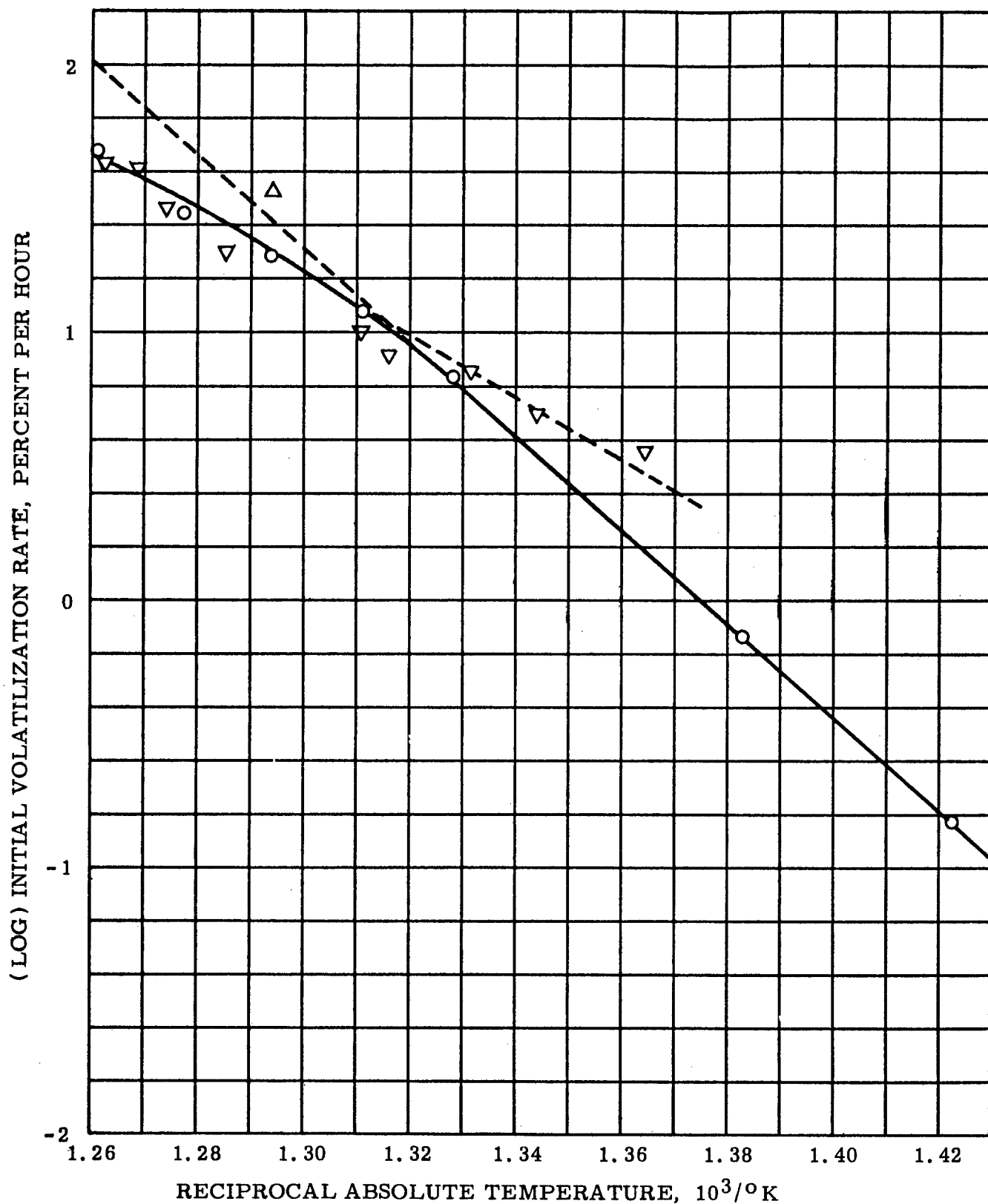
Figure 23 COMPARISON OF VOLATILIZATION RATES FROM THE MAGNIFIED THERMOGRAM "▽" WITH INITIAL VOLATILIZATION RATES FROM ISOTHERMAL AGING OF POLYTETRAFLUOROETHYLENE IN DRY N 2 , "○" AND IN VACUO "Δ"
