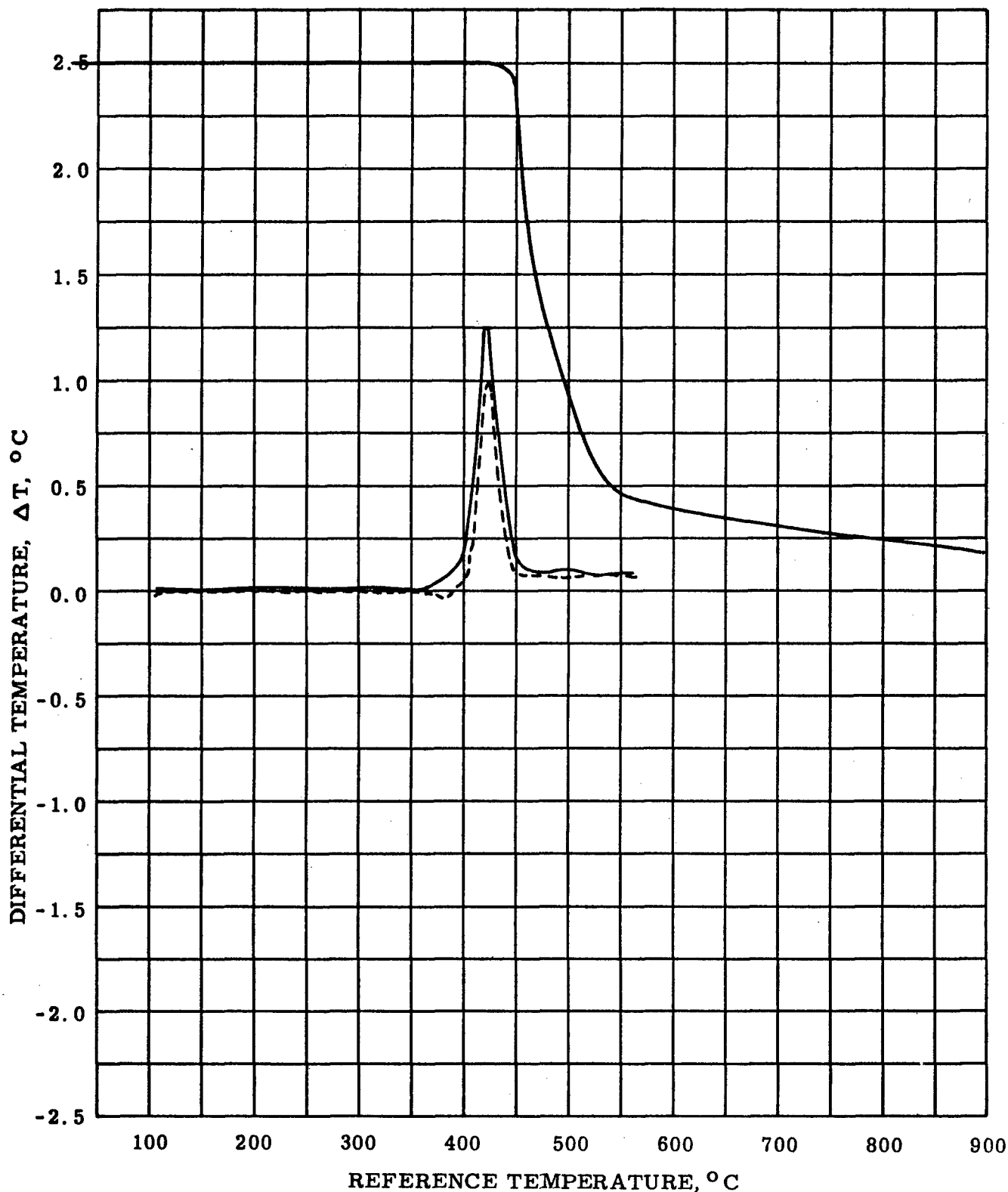
Figure 47 DTA IN DRY N_2 AT 180\text{ }^\circ\text{C}^\circ PER HOUR, COMPARED WITH TGA AT THE SAME HEATING RATE, ZINC 4, 4' - BIS - THIOPICOLINAMIDODIPHENYL
