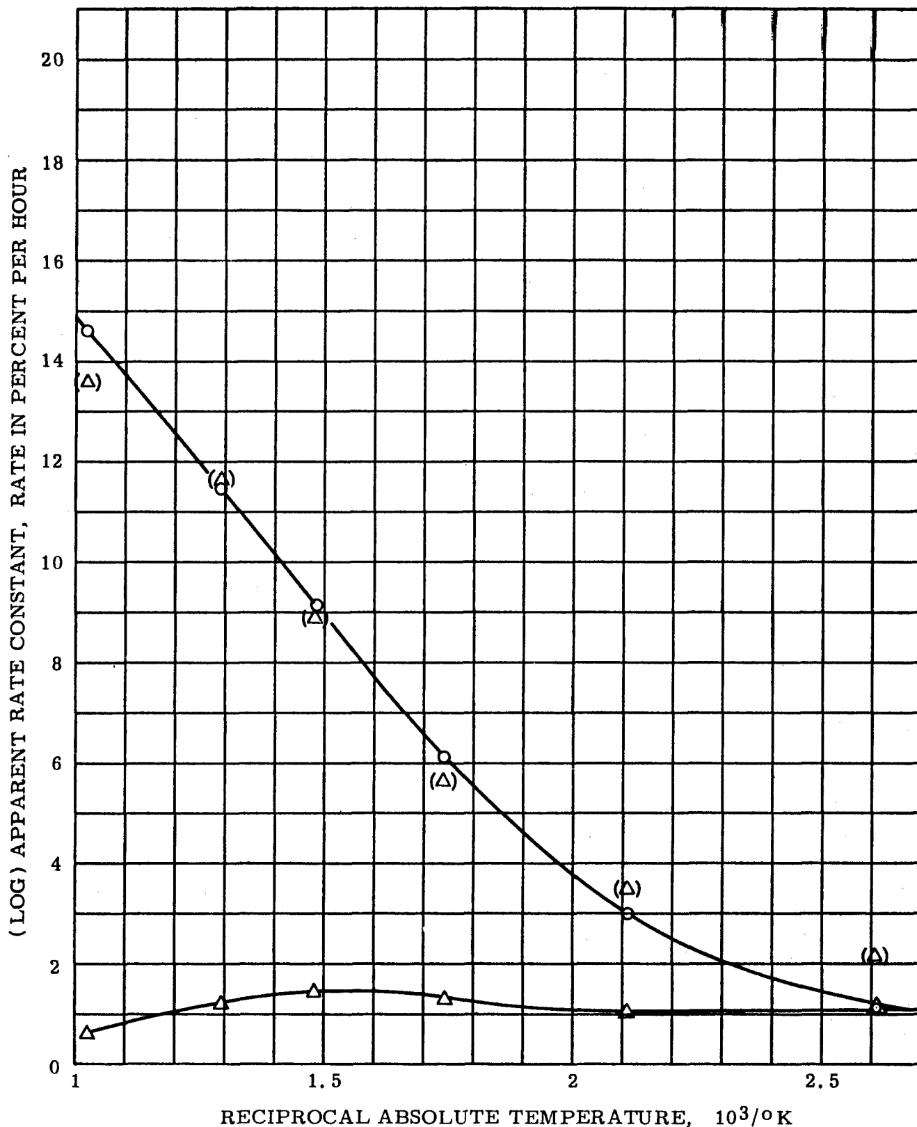
Figure 35 COMPARISON OF VOLATILIZATION RATES, " \Delta " AND ESTIMATED APPARENT RATE CONSTANTS, " \Delta " FROM THE MAGNIFIED THERMOGRAM WITH APPARENT RATE CONSTANTS, "O" FROM ISOTHERMAL AGING OF THE REACTION PRODUCT OF ACONITIC ACID AND ACETIC ANHYDRIDE, CODE 88, 8/58, IN DRY \text{N}_2
