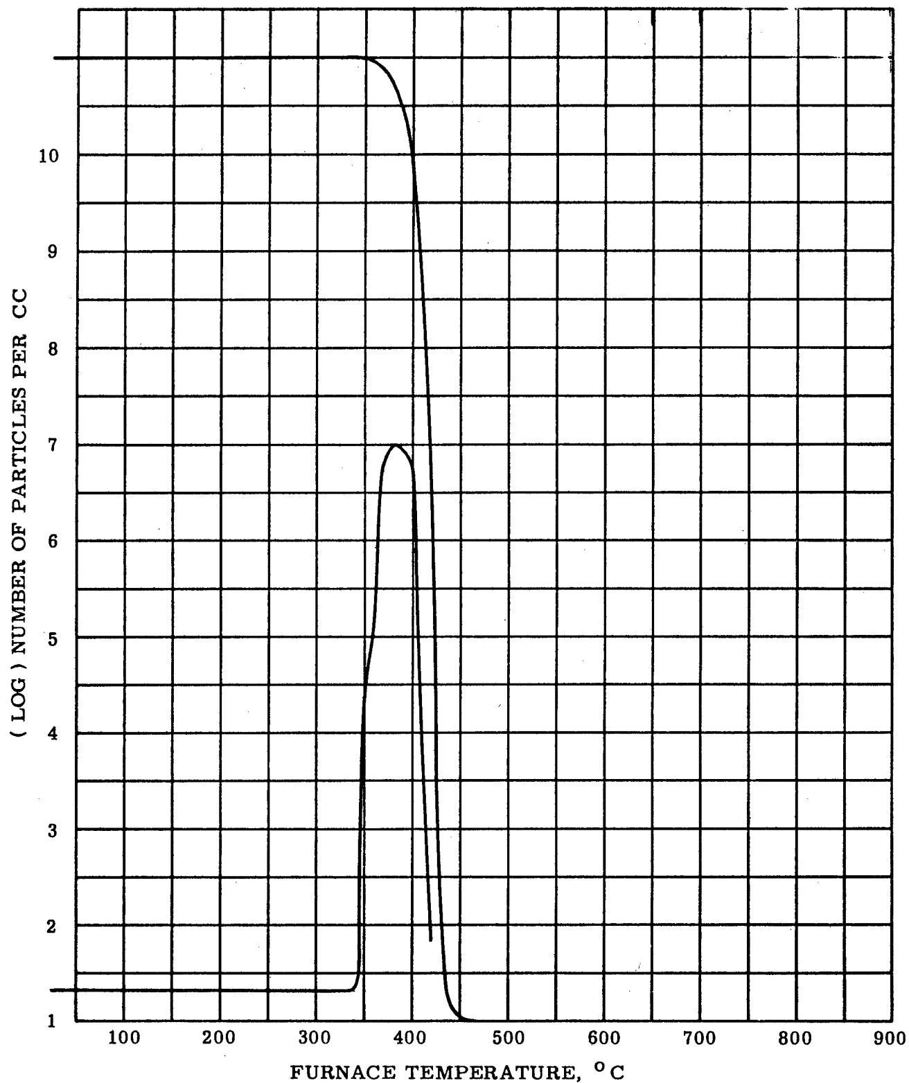
Figure 57 TPA IN DRY N_2 AT 180^\circ C PER HOUR, COMPARED WITH TGA AT THE SAME HEATING RATE, POLYCHLOROTRIFLUOROETHYLENE
