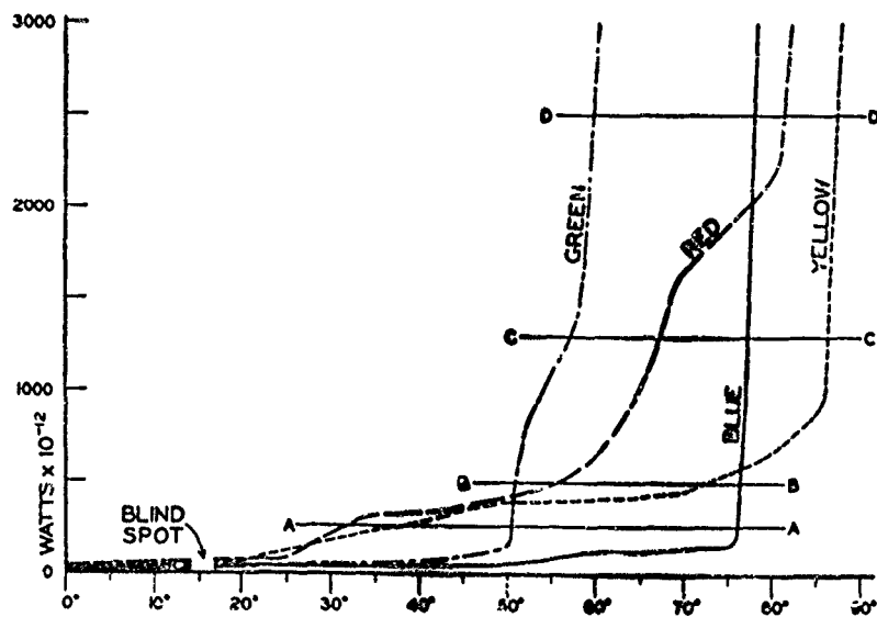
Figure 1 Color zone size as a function of energy (Data of Ferree and Rand, Psychol. Rev. , 1919, 26, 16-41. Reproduced from Boring, 1942.)
