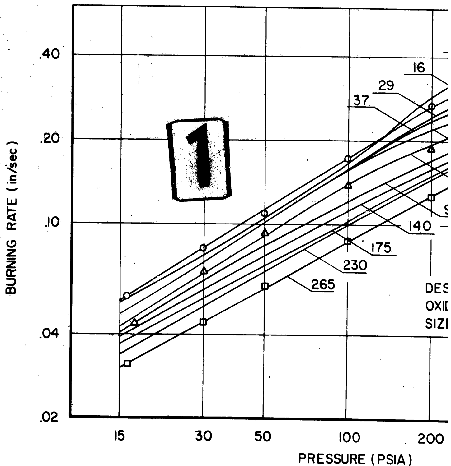
FIGURE 2 BURNING RATE VS P POLYSULFIDE PROPELLANTS, NARROW PARTICLE SIZE DISTRIBUTION
