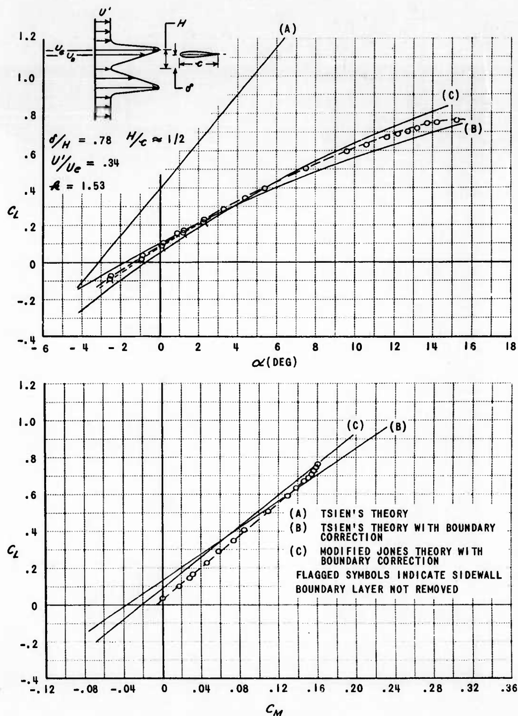
Figure 19d LIFT AND MOMENT IN A TWO-DIMENSIONAL SLIPSTREAM WITH LARGE SHEAR
