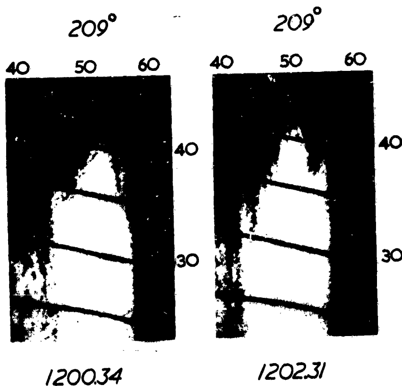
FIG. 39 Full-gain 3.3 cm RHI photographs along 209^\circ at 1200.34 and 1202.31 to show a top at range 56 miles moving with a component velocity along this azimuth of only 15 mi/hr.
