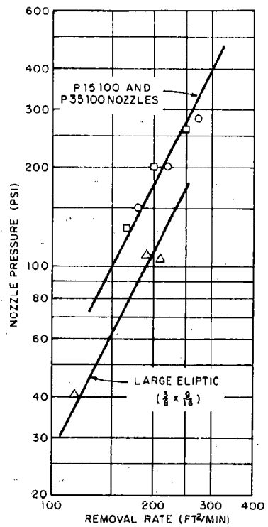
Fig. A.5 Performance Curves for Water Broom Nozzles
