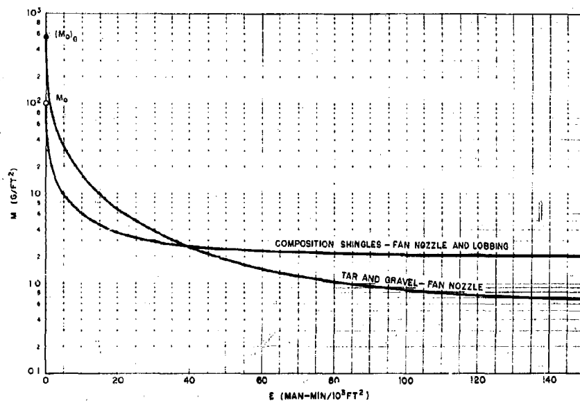
Fig. 4.2.3 Comparative Effectiveness of Decontamination Methods on Roofs for an M_0 of 100 \text{ g/ft}^2
