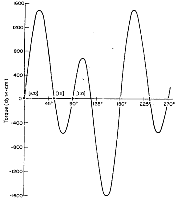
Fig. 19. Torque vs. angle curve for nickel in the (110) plane at 20^\circ\text{C} .
