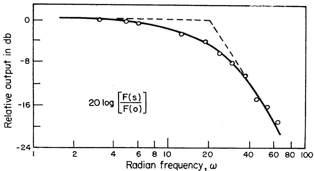
Fig. 13. Amplifier-response curve.
