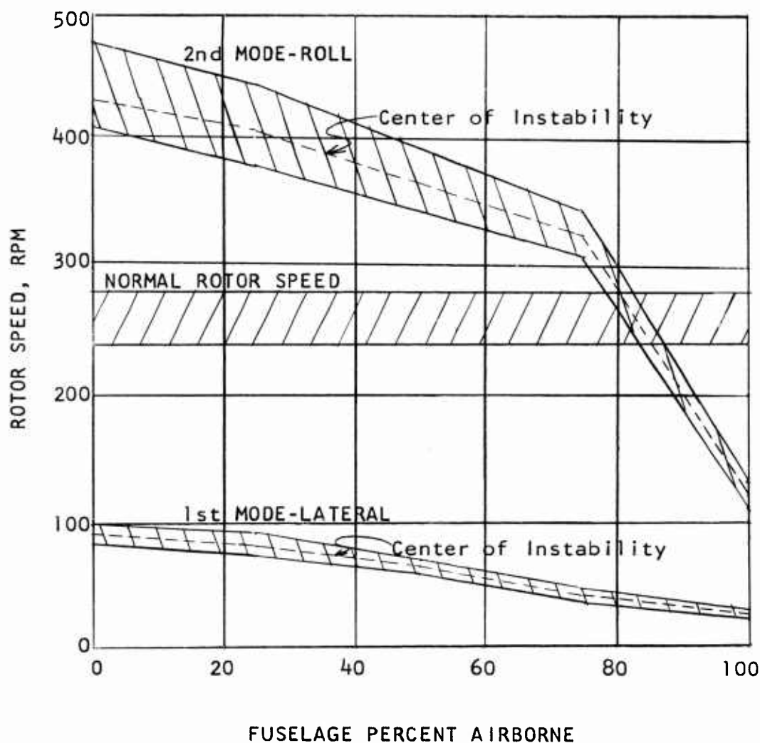
INSTABILITY REGION vs. AIRCRAFT ATTITUDE
