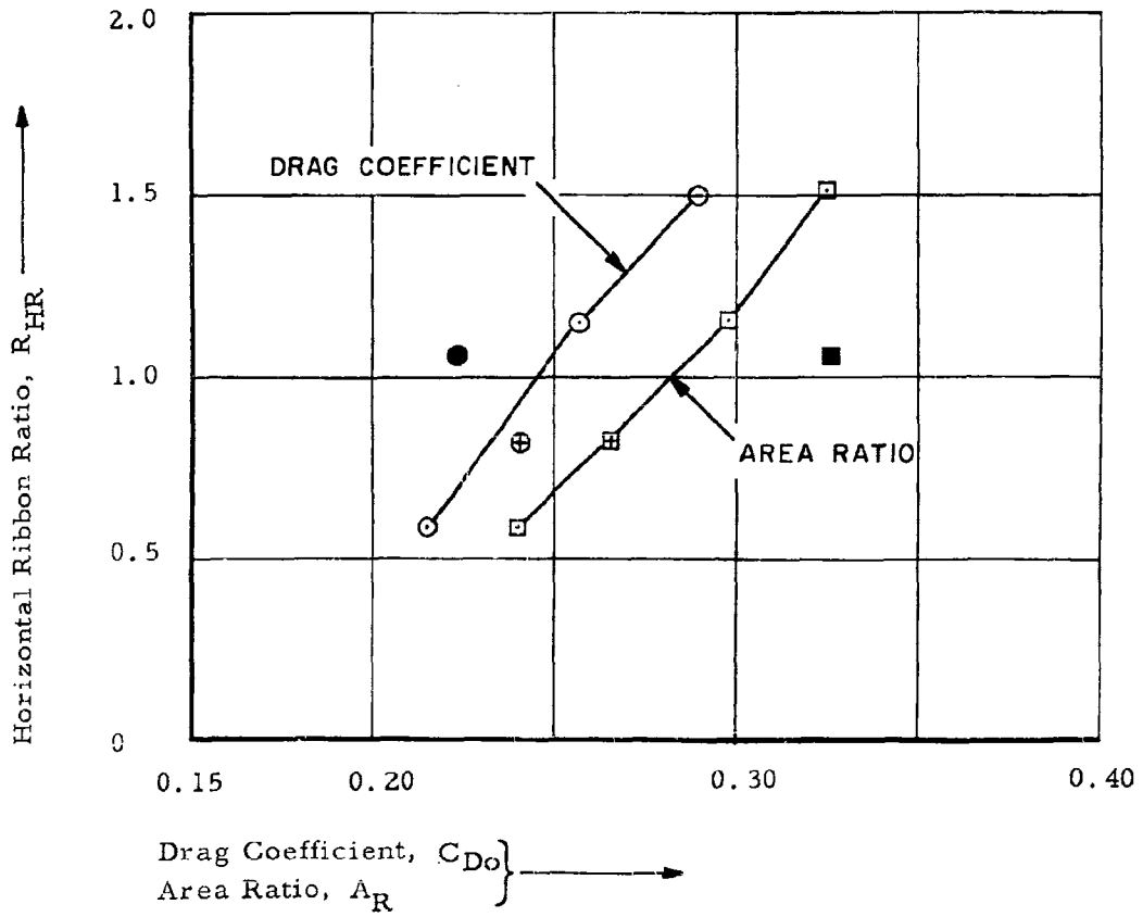
Figure 12. Horizontal Ribbon Ratio vs. Drag Coefficient and Area Ratio for 16 Gore Model Parachutes at Mach 1.9
