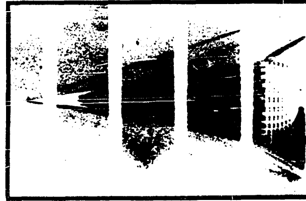
(b) Mach No. = 3.71 Dynamic Pressure = 200 P.S.F. Suspension Lines = 24 x 2D Film Speed = 480 F.P.S.
