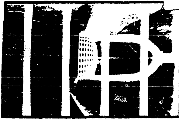
(a) Porosity = 28% Mach No. = 1.77 Dynamic Pressure = 290 P.S.F.
