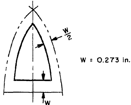
CRITICAL GORE CONFIGURATION
