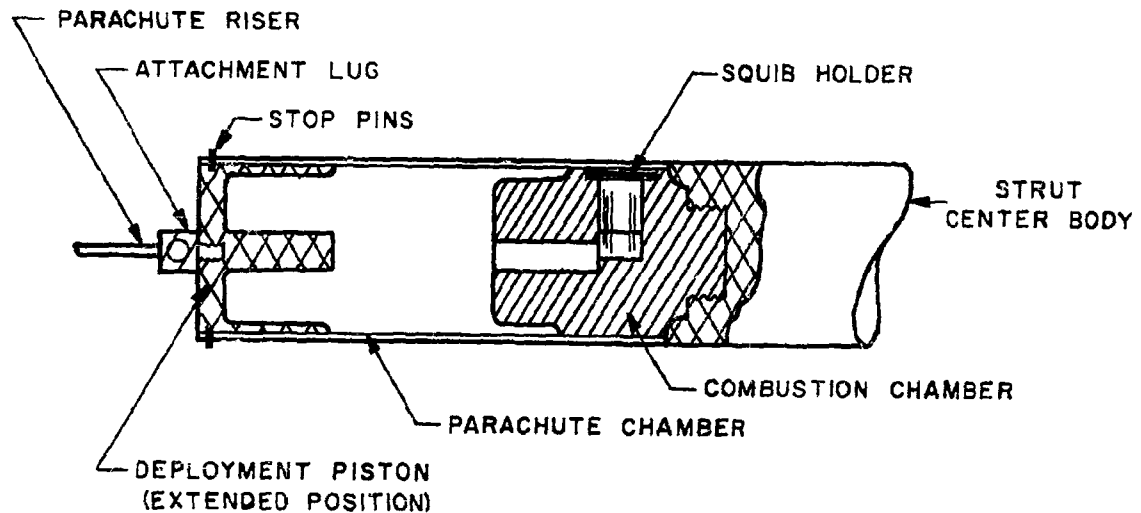
SCHEMATIC DIAGRAM OF THE DEPLOYMENT MECHANISM
