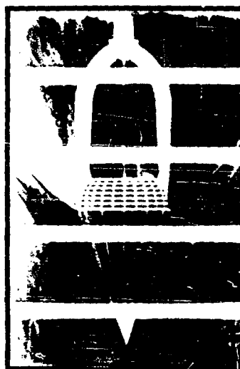
(b) Mach No. = 2.17 Dynamic Pressure = 240 P.S.F. Film Speed = 2040 F.P.S.
