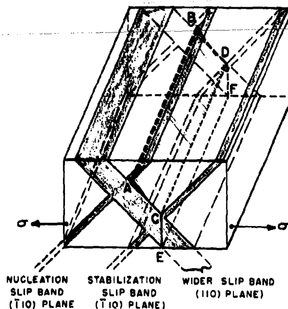
Figure 7 - Formation of cracks at slip band intersections. Crack nucleates along AB, propagates by cleavage over \langle 110 \rangle and is then stabilized along CD to form a slit ABCD.
