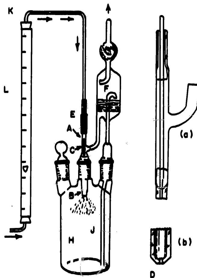
Figure 18. Ozone-Absorbing Device.
