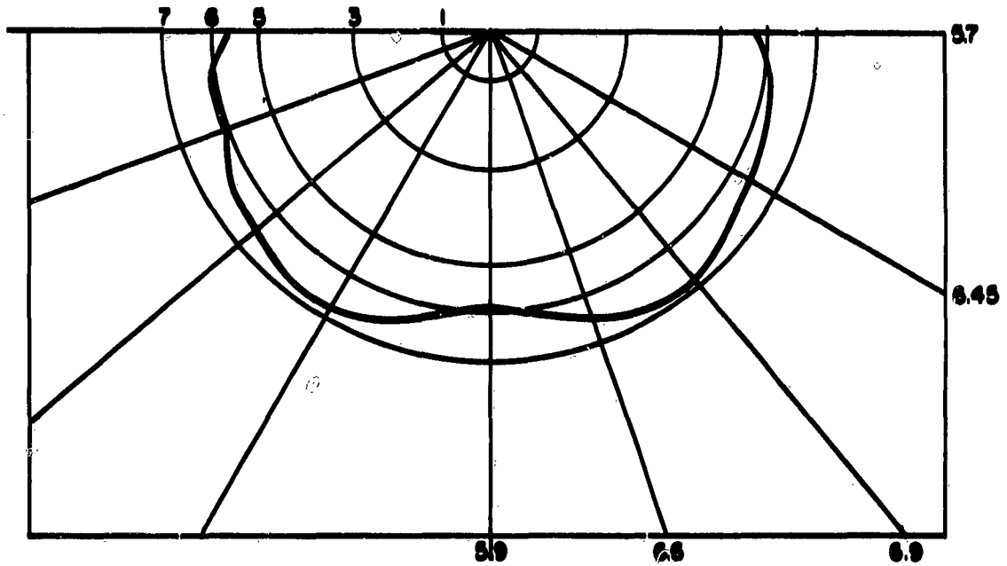
Figure 9. Distribution from a Cold Cathode Lamp (782-30) Installed in a SB-30 Fixture.
