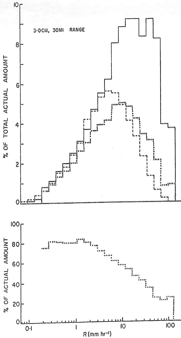
FIG. 15. Above: Rainfall amount as a function of rainfall rate. Below: Ratio of apparent rainfall amount (dotted curve above) to actual rainfall amount (solid curve above) as a function of rainfall rate.
