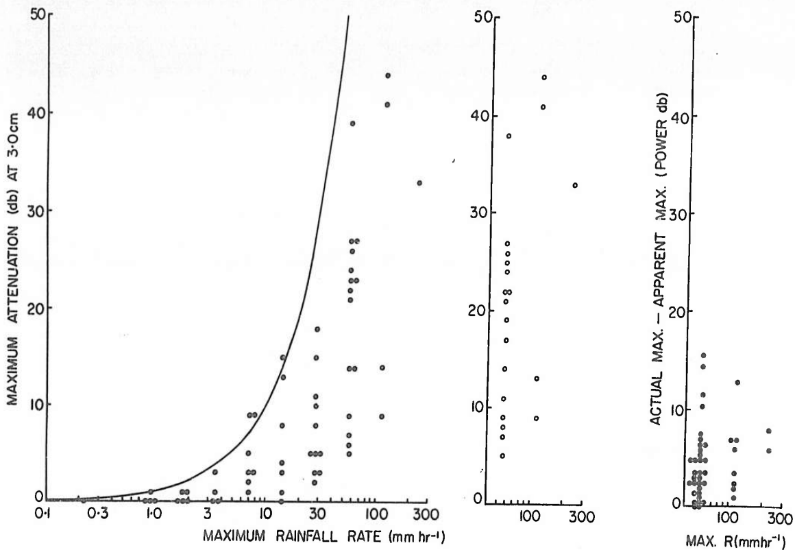
FIG. 11. The maximum attenuations of parts (a) and (b) are much greater than the amount by which the apparent maxima fall below the actual.
