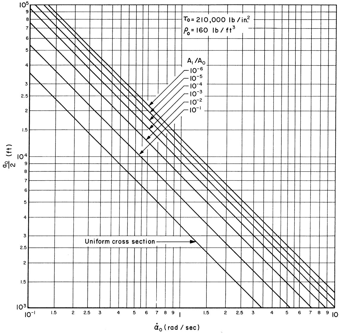
Fig.4- Length of wire vs angular rate
