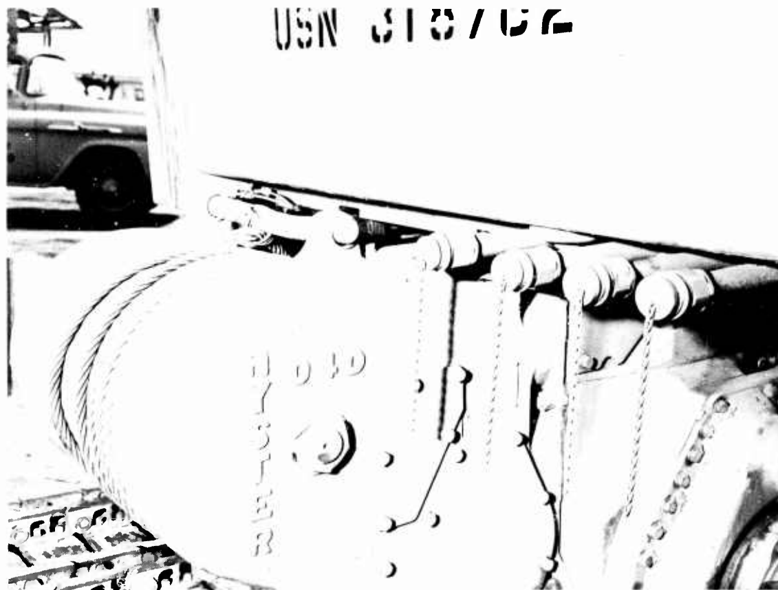
Figure 17. Hydraulic power take-offs at rear of low-ground-pressure snow tractor.
