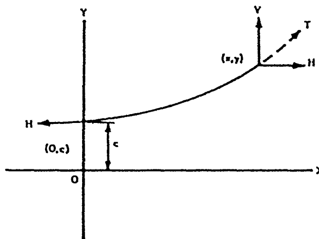
Figure C-1. Catenary curve.
