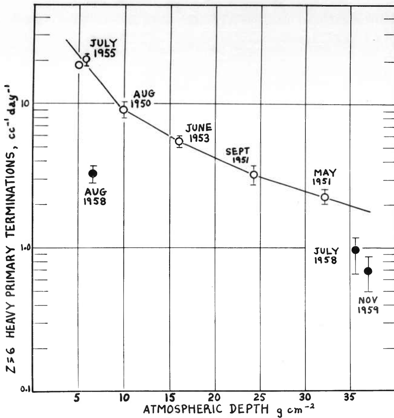
FIG. 6. Comparison of thindown frequencies in emulsions flown in the stratosphere during periods near maximum and minimum sunspot activities, at geomagnetic latitudes of about 55^{\circ}N .
