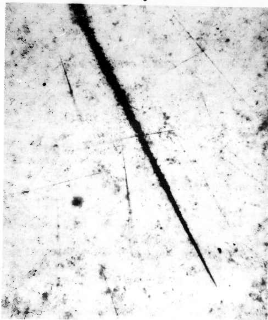
Fig. 1. Terminal portion of a heavy primary nucleus of charge Z = 23 \pm 3 exhibiting characteristic tapering of the track as the particle reaches the end of its range. The track is 600 microns long.
