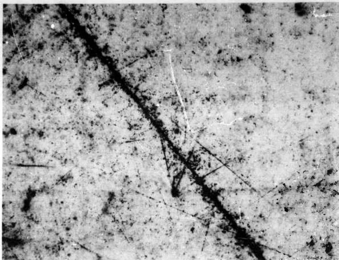
Fig. 5. Photomicrograph of a five-prong star produced by the disintegration of a silver or bromine atom in the emulsion as a result of interaction with a secondary cosmic-ray neutron. The heavy track was produced by the same particle whose terminal portion is shown in Fig. 1. The particular focal setting is at 35.6 mm from the end of the range, corresponding to a kinetic energy of 290 BEV.
