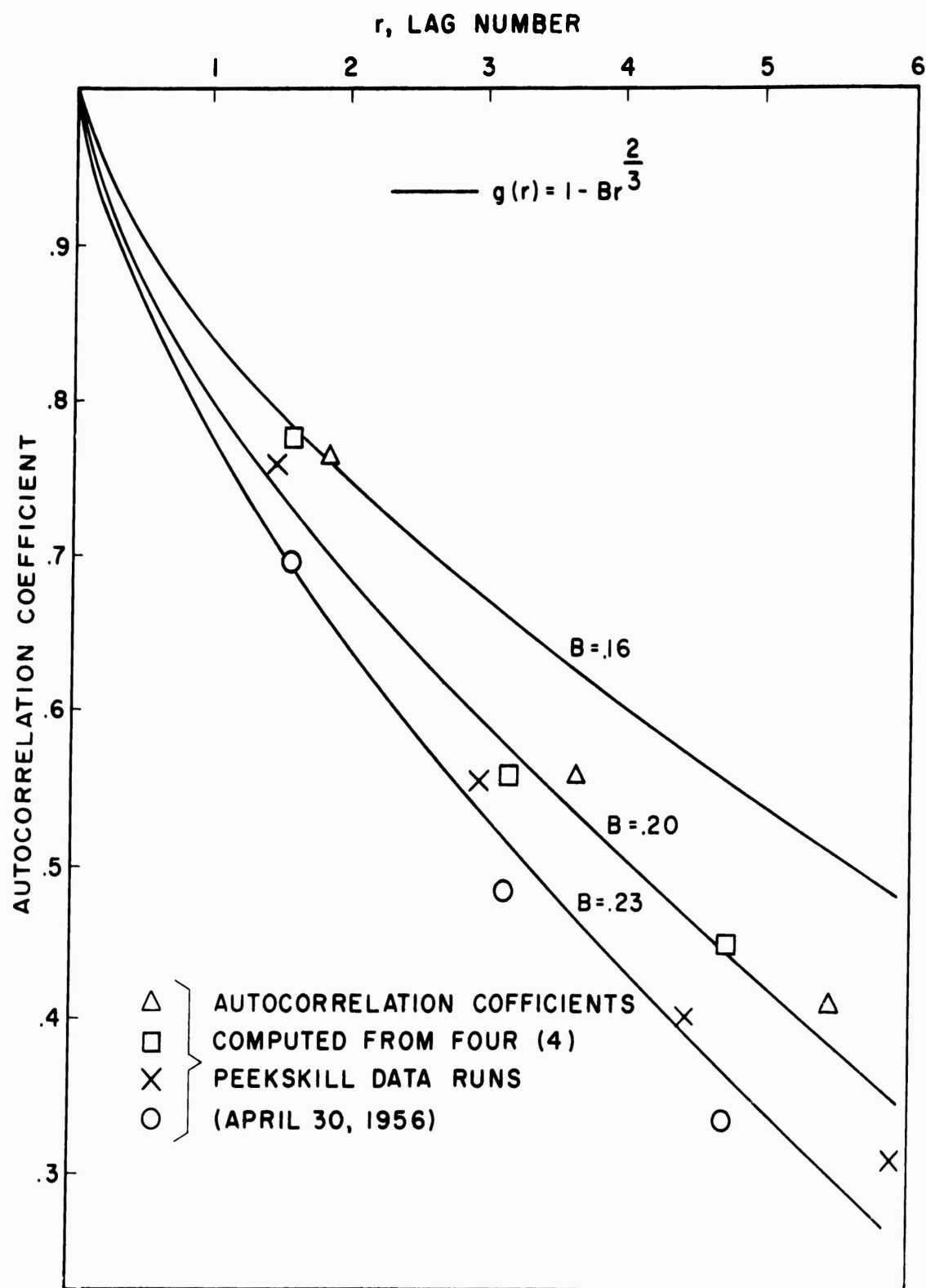
FIGURE II PEEKSKILL TOWER DATA COMPARED WITH CORRELATION FUNCTIONS CORRESPONDING TO -\frac{5}{3} POWER LAW.
