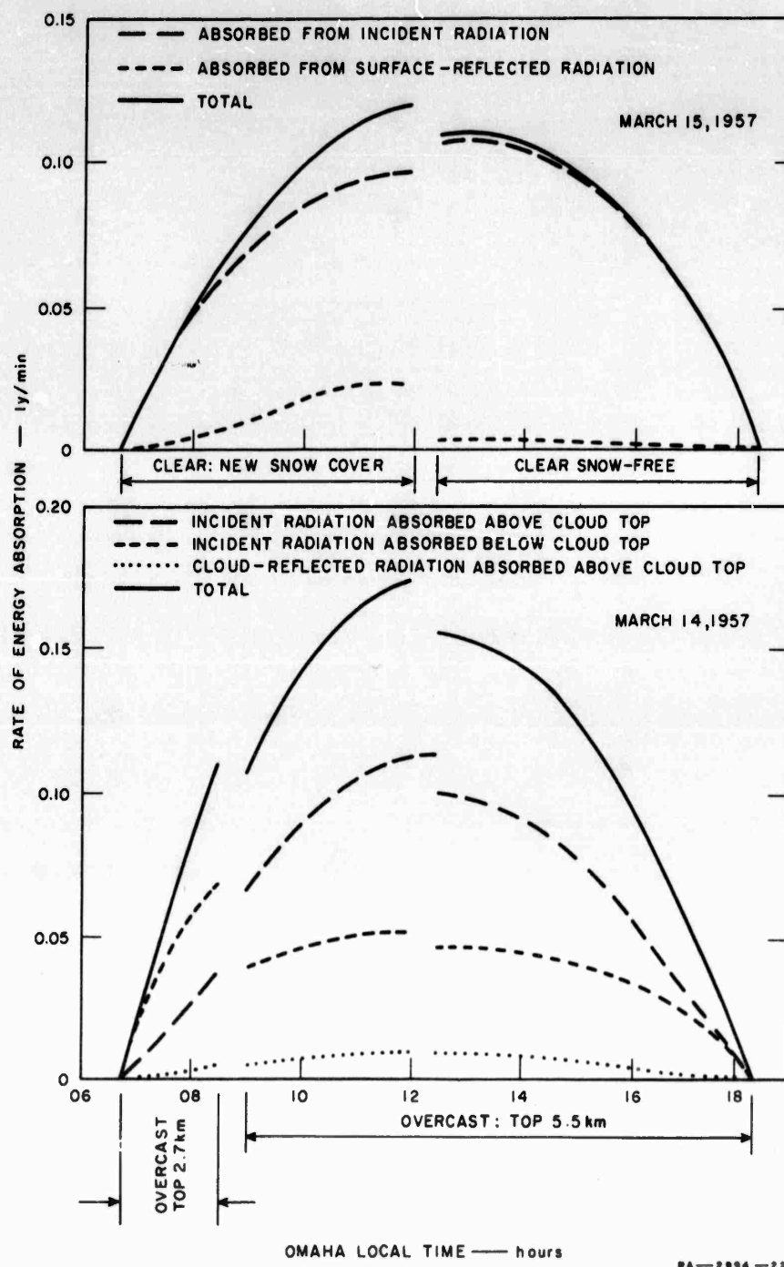
FIG. 17 RATE OF SOLAR ENERGY ABSORPTION BY ATMOSPHERIC WATER VAPOR AT OMAHA AS A FUNCTION OF LOCAL TIME FOR SELECTED SYNOPTIC SITUATION
