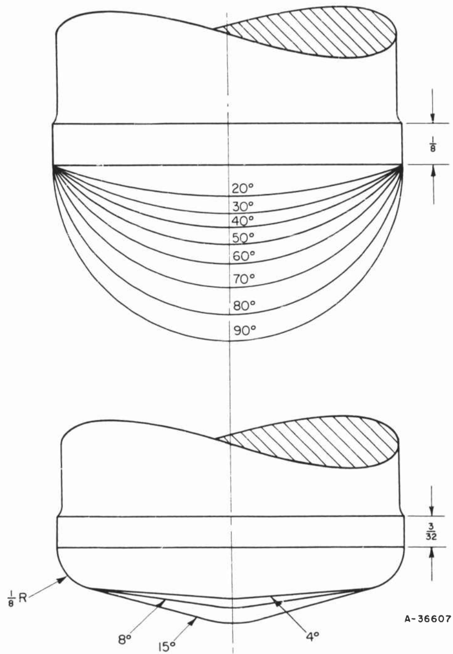
FIGURE 5. PUNCH-TIP CONFIGURATIONS STUDIED IN BACKWARD-EXTRUSION EXPERIMENTS
