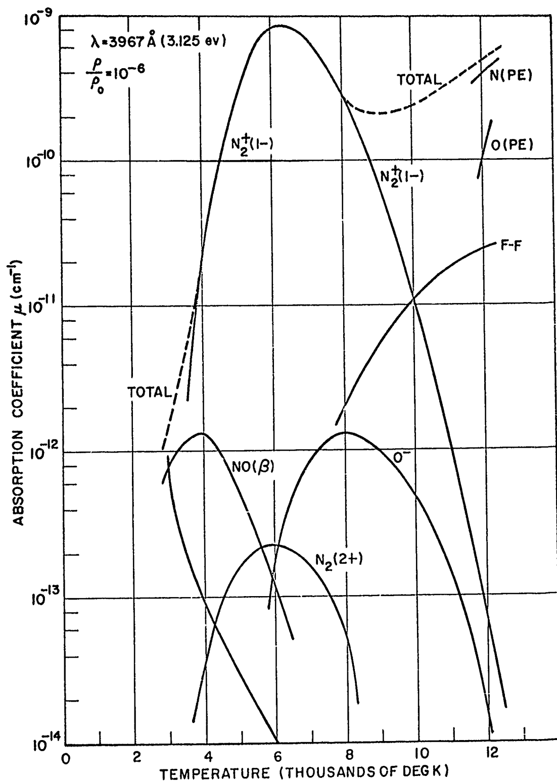
Fig. 10 Absorption Coefficient for \lambda = 3967 \text{ \AA} , \rho/\rho_0 = 10^{-6}
